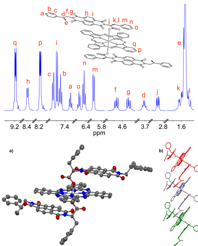
Figure 1. Top: the structure and labelled 1 H NMR spectrum of Pc8 in \text{CDCl}_3 at room temperature. Bottom: a) ORTEP representation of Pc8 . The thermal ellipsoids were drawn at 50% probability level (Hs were removed for clarity); b) fragment of the extended aromatic \pi - \pi stacking in the crystal packing of Pc8 .
