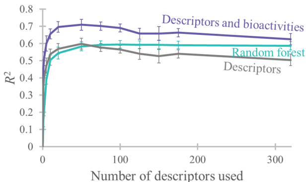
Figure 3: The coefficient of determination for predicting the activity of the adrenergic receptors with number of chemical descriptors. The magenta line is when the neural network is trained with both the activities and descriptors present, the grey line with just the descriptors, and the cyan line is for random forest. Error bars represent the standard error in the mean R^2 over five-fold cross-validation.
