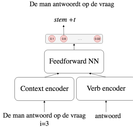
Figure 1: Architectural overview of the dt-corrector. The input to the system is the position of the verb i and the sentence where the input verb is replaced by its stem. Two neural networks are responsible for encoding the representations of the context and the verb respectively. The resulting representations are concatenated and fused by a feed-forward neural network and transformed to a probability distribution over suffixes using a softmax layer.
