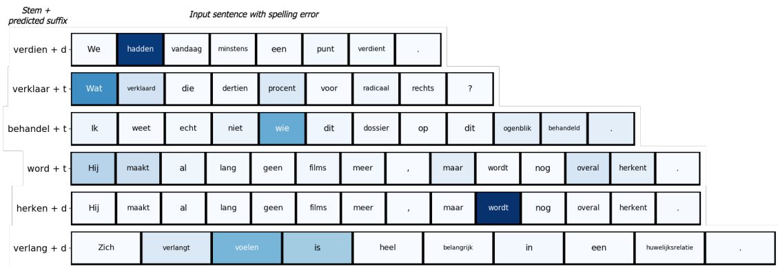
Figure 3: Heatmaps of the impact of each word on the prediction of the neural network for wrongly spelled dt-verbs from the De Standaard test set. Impact of a word is measured by the decrease in probability mass of the predicted class when we mask the word in the context encoding (i.e., replace its word embedding by a vector of zeros).
