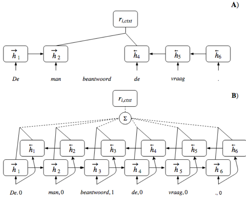
Figure 2: Illustration of the context encoders: A) BiLSTM, B) BiLSTM + ATTENTION
