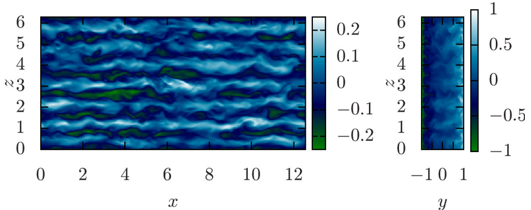
FIGURE 2. Streamwise velocity, u , for the case Re = 5000 , F_h^{-2} = 0.1 , Pr = 1 , L_x = 4\pi , L_z = 2\pi from set 1 of DNS in table 1. Left panel shows the flow at the mid-gap y = 0 and the right panel shows the flow for x = 0 . Seen are the streaks of high/low speed fluid which have been lifted from near the walls by streamwise rolls, as one expects in plane Couette flow. In these images there is no discernible effect of stratification on the dynamics.
