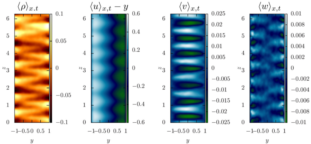
FIGURE 5. Streamwise- and time-averaged total velocities \langle \mathbf{u} \rangle_{xt} - y\hat{\mathbf{x}} for Re = 5000 , F_h^{-2} = 0.1 , Pr = 1 , L_x = 4\pi , L_z = 2\pi from set 1 of DNS in table 1. Streamwise vortices emerge as a coherent structure coupled to the density layering.
