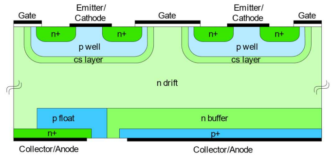
Fig. 7. CSFP-RC-IGBT structure [31].
