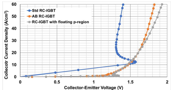
Fig. 9. I-V characteristic of AB RC-IGBT ( L_C (collector length) =30\mu\text{m} , L_P (p+ length) =25\mu\text{m} ), RC-IGBT with floating p-region ( L_C=30\mu\text{m} , L_P=25\mu\text{m} ) and a conventional RC-IGBT ( L_C=300\mu\text{m} , L_P=295\mu\text{m} ) [32].
