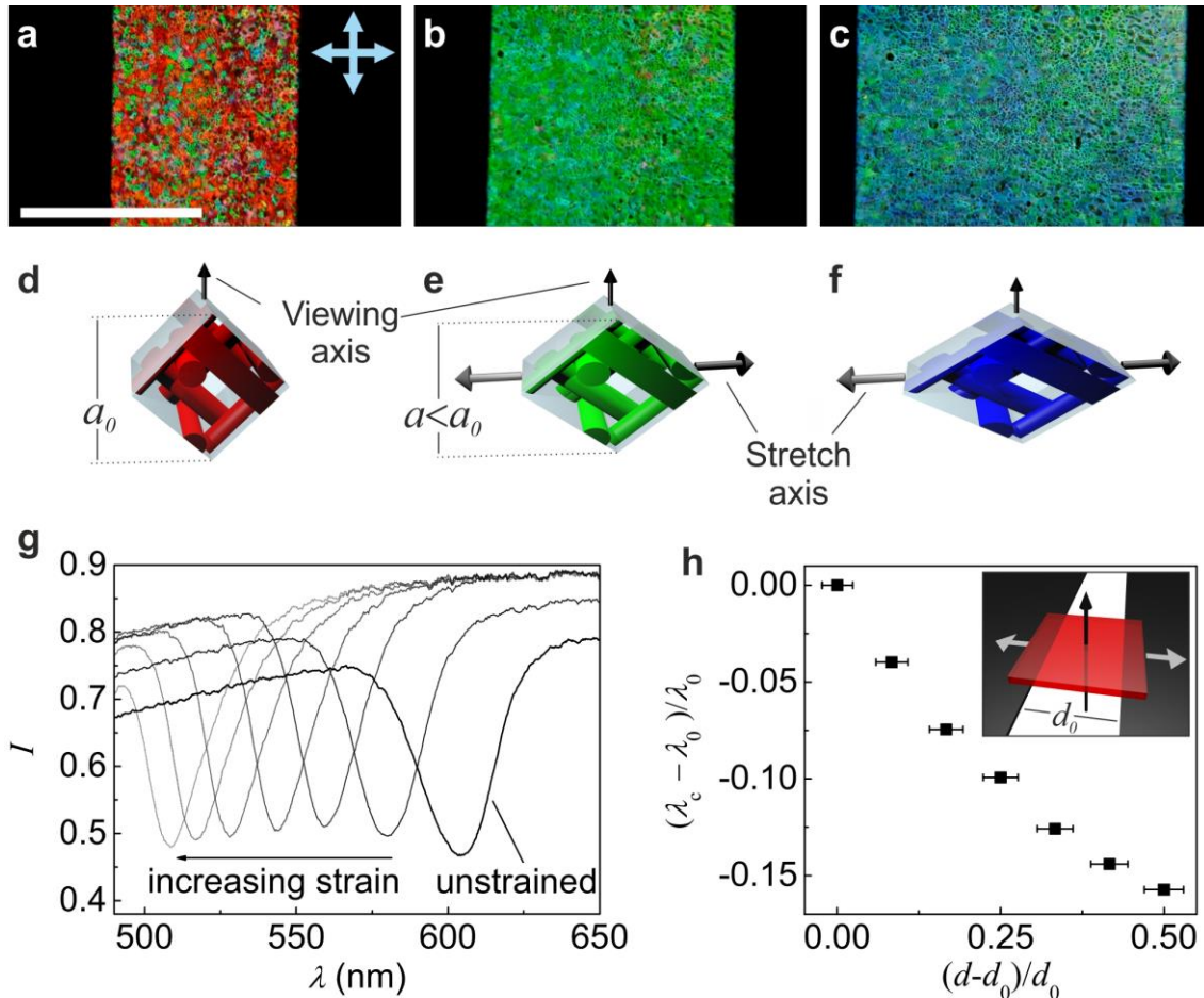
Figure 2 | Colour changes in a stretchable blue phase gel. a, b & c , Polarizing optical microscope images of a 20 \mu\text{m} thick layer placed across a variable-width aperture. The un-stretched state, a , displays a characteristic blue phase texture. Pale blue arrows denote the orientation of the crossed polarisers (scale bar, 1 mm). As the aperture is widened, b & c , the sample is stretched and a colour change induced. d, e & f , Schematic diagram of a typical deformation of the blue phase I unit cell, viewed along the [011] direction and stretched along an axis perpendicular to this. g , Spectral analysis of a sample with uniformly aligned [011] platelets showing the relative transmitted intensity I as a function of the vacuum wavelength of transmitted light \lambda . Curves with reflection bands from right to left correspond to aperture widths in this experiment of 0.60 mm (unstrained), 0.65 mm, 0.70 mm, 0.75 mm, 0.80 mm, 0.85 mm, and 0.90 mm respectively. h , The wavelength of maximum selective reflection \lambda_c , defined as the minimum of I(\lambda) , is plotted as a function of the aperture width d , normalised by the values in the initial, unstrained, state \lambda_0 and d_0 . The random uncertainty in a measurement of d was estimated from the graduation on the screw gauge to be \pm 0.01 mm, and the random uncertainty in the measurement of \lambda_c was negligible in relation to this. Inset: schematic diagram showing the geometry of the experimental setup.
