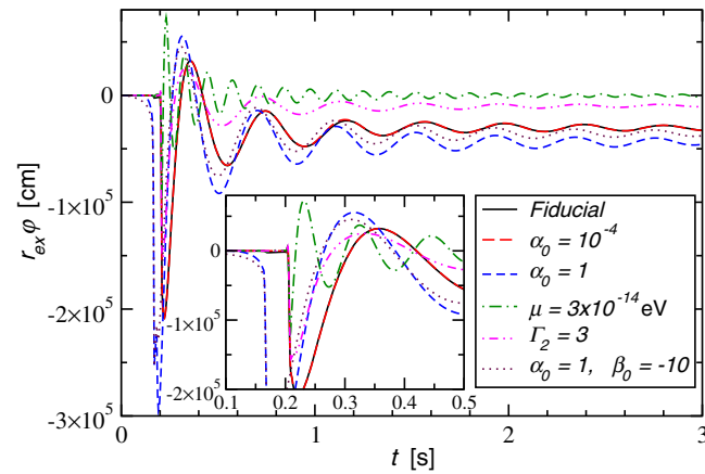
FIG. 1. Waveforms extracted at 5 \times 10^4 km. The legend lists deviations from the fiducial parameters \mu = 10^{-14} eV, \alpha_0 = 10^{-2} , \beta_0 = -20 , \Gamma_1 = 1.3 , \Gamma_2 = 2.5 , and \Gamma_{\text{th}} = 1.35 .
