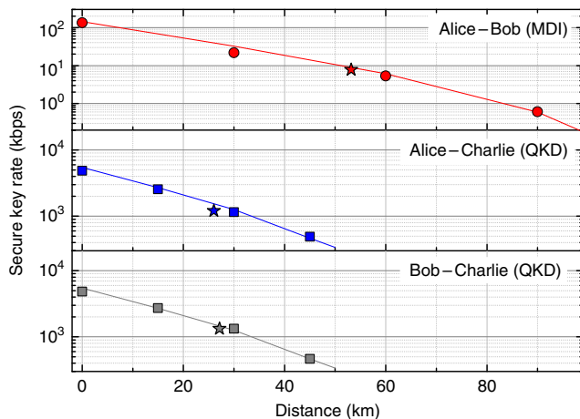
Fig. 3 Secure key rates vs. distance. MDI-QKD (top diagram) and QKD (centre and bottom diagrams) secure key rates for a Z (X) basis probability equal to 80% (20%) and a security parameter \epsilon_{\text{sec}} \lesssim 10^{-10} are shown as a function of distance. Because the reconfigurable scheme is symmetrically deployed, the distance between Alice and Bob (top) is approximately twice the distance between Alice and Charlie (centre) and Bob and Charlie (bottom). All the distances have been calculated assuming 0.2 dB/km attenuation on the channel, except for the data points indicated by stars, where a real fibre was used. The projected time to attain the shown key rates is 25 h of which 3 min are spent on QKD and the rest on MDI-QKD, to balance their key rates. The fitting lines are the result of a numerical simulation with the parameters mentioned above and the following additional ones: Charlie’s insertion loss, 1.1 dB; detectors’ efficiency and temperature, 20% and 0°, respectively; afterpulsing, 4%; dark count probability per gate, 1.6 \times 10^{-5} ; error correction coefficient, 1.16
