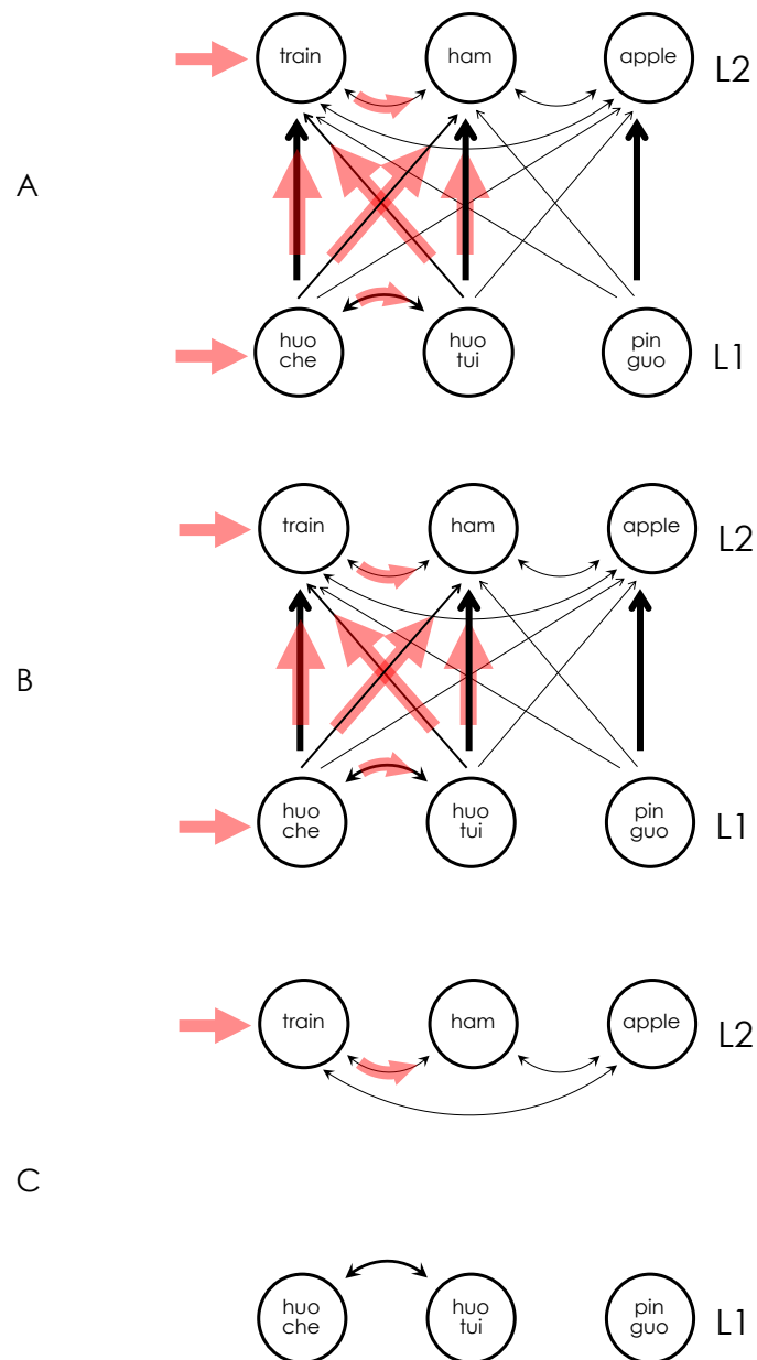
Figure 1 – Schematic of the cross-linguistic pattern-completion model as implemented in Costa et al.’s L1-connected simulation (A), their L1-disconnected simulations (B), and our L1-fully-disconnected simulation (C). Line thickness approximates connection strength on a logarithmic scale, completely omitting connections of weight 0. Overlays depict activation flow through major connections supporting ‘ham’ over ‘apple’. Panels A and B are identical because Costa et al.’s L1 disconnection only removed connections from L2 to L1, which never actually developed in the first place.
