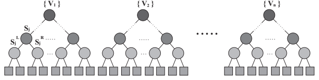
Figure 6. Random Forests
