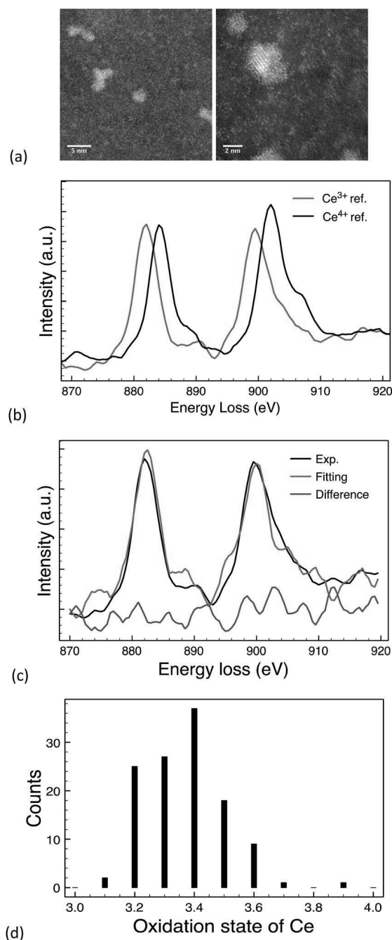
Fig. 6 (a) STEM images for 10k PVP capped ceria, (b) reference EELS spectra of commercially available \text{Ce}^{3+} ( \text{Ce}(\text{NO}_3)_3 salt); and \text{Ce}^{4+} ( \text{CeO}_2 NMs) materials; (c) MLLS fitting of an EELS spectrum from one \text{CeO}_x NM; & (d) oxidation state distribution of \text{CeO}_x NPs.
