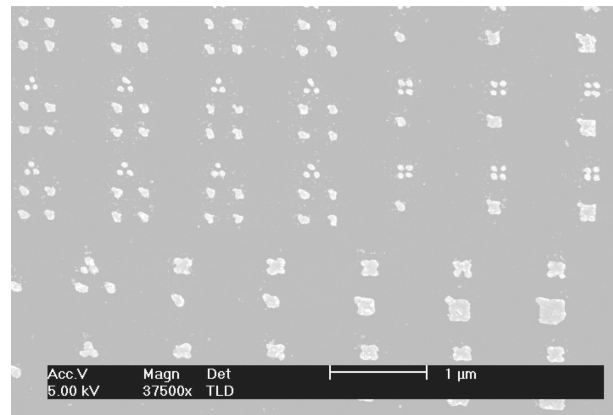
Figure 2. Scanning electron micrographs of 30 nm thick Ag nanostructure array produced on HOPG by electron-beam lithography.
