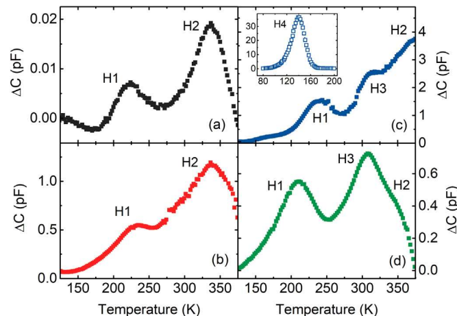
Fig. 8. DLTS spectra recorded for samples with various bulk As concentrations: (a) 1 \times 10^{16} , (b) 3 \times 10^{17} , (c) 4 \times 10^{18} , and (d) 1 \times 10^{19} \text{ As cm}^{-3} . Spectra were recorded over a 125–375 K range with a 2 K increment using a pulse width of 0.1–100 ms depending on the sample. Inset to (c) shows the low temperature (80–200 K) DLTS spectrum recorded for 4 \times 10^{18} \text{ As cm}^{-3} using a pulse width of 1 \mu\text{s} . Positions of observed hole (H) trap levels are labelled.
