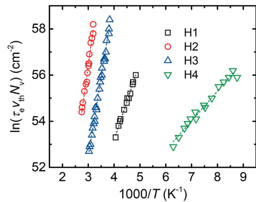
Fig. 9. Arrhenius plots of defect levels observed in DLTS spectra. Trap energy is derived from the slope with capture cross section determined from the intercept with the \ln(\tau_e V_{th} N_V) axis.
