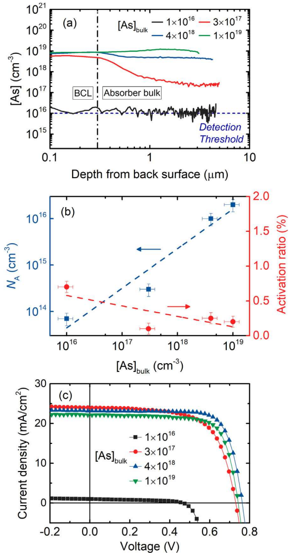
Fig. 3. (a) SIMS As concentration [As] depth profile and (b) acceptor density and activation ratio of the absorber in the CdTe:As solar cells studied. The \sim 1 \times 10^{16} As \text{cm}^{-3} sample is unintentionally-doped and does not contain the heavily-doped ( \sim 1 \times 10^{19} As \text{cm}^{-3} ) back-contact layer. (c) Typical light J - V curves of the CdTe:As solar cells.
