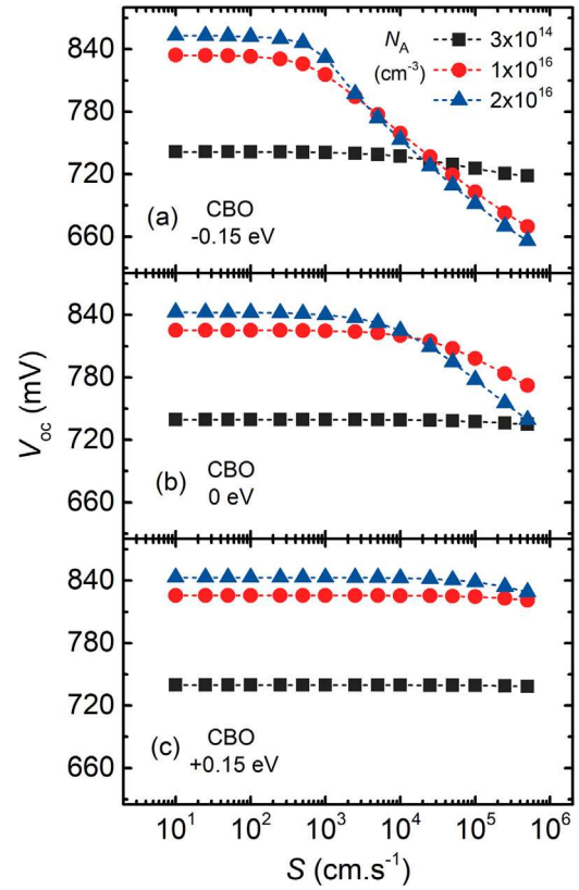
Fig. 6. V_{oc} vs. interface recombination velocity ( S ) between CdZnS and CdTe layers for varying acceptor concentration ( N_A ) and for three different conduction band offset ( \chi_{\text{CdTe}} - \chi_{\text{CdZnS}} ) values of (a) CBO = -0.15 eV, (b) CBO = 0 eV, and (c) CBO = +0.15 eV. A small positive CBO, i.e. spike, is beneficial for maintaining the V_{oc} when S \geq 10^3 - 10^4 \text{cm s}^{-1} .
