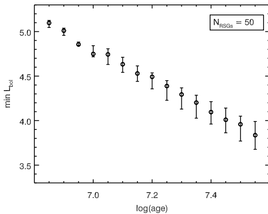
Figure 3. Plot showing the most likely RSG L_{\min} for a cluster at a given age containing 50 RSGs, from MIST non-rotating isochrones (Dotter 2016). Each point represents the median L_{\min} of 1000 trials while the error bars represent the 68% probability limits. For clusters with fewer RSGs the relation stays the same but there are more stochastic errors.
