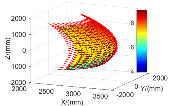
(b) Cutting-head position error distribution when the external parameter calibration error is set at 0.1^\circ
