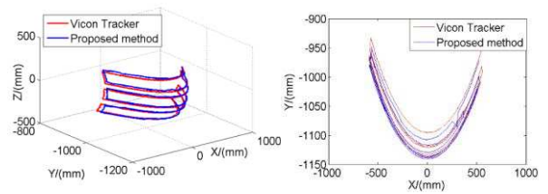
(a)The trajectory of the cutting-head when its move in the S-shaped motion path; (b)The trajectory of the cutting-head projected in the XY plane;
