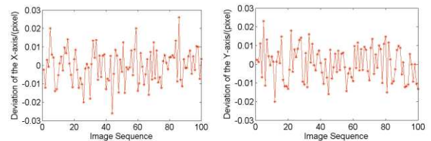
(a)Deviation of the X-axis (b)Deviation of the Y-axis
