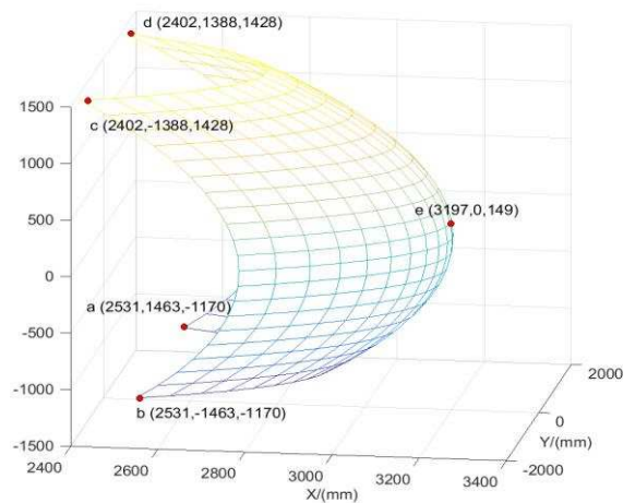
(a)The five extreme positions of cutting face
