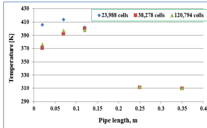
Fig. 6 Temperature distributions along the length of the thermosyphon for different mesh sizes
