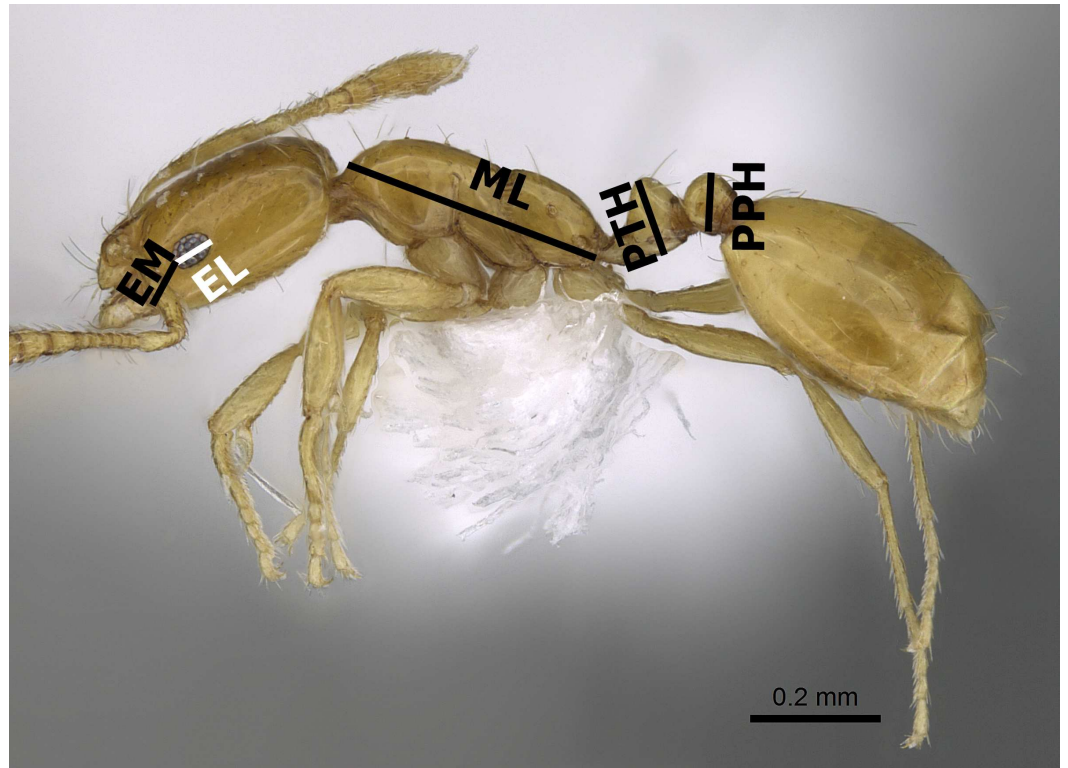
Figure 1 Body profile of M. exiguum Forel (CASENT0922302, from https://www.antweb.org/specimenImages.do?name=casent0922302&countryName=South%20Africa —Michele Esposito) illustrating the used measurements.
