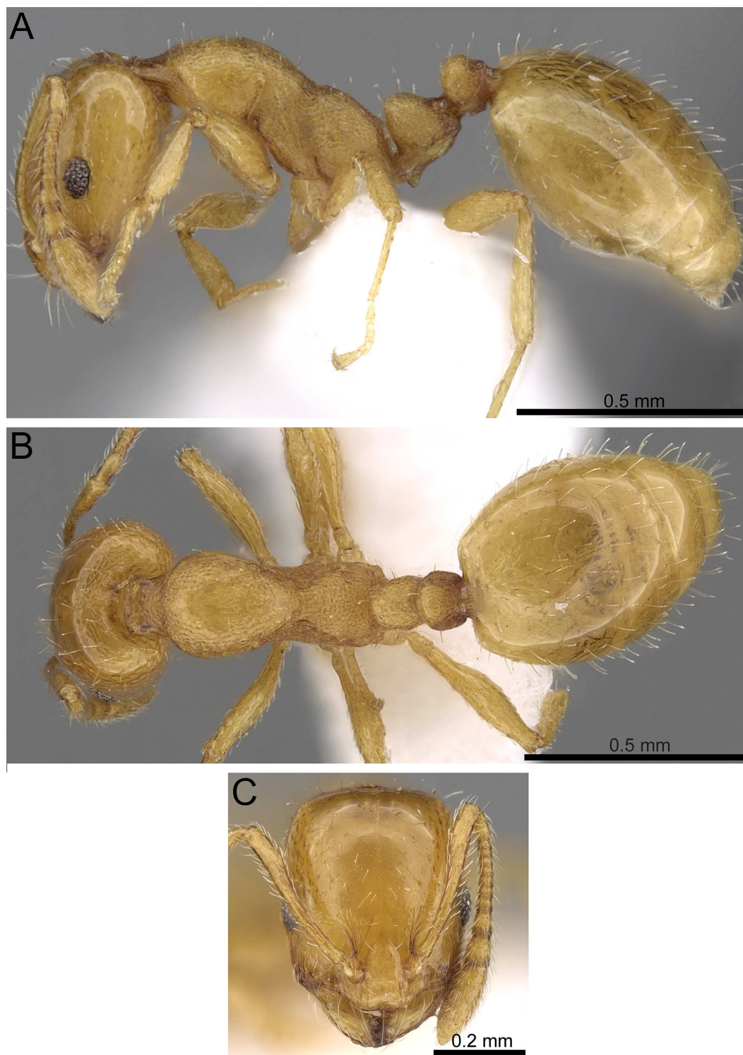
Figure 10 Monomorium sarawatense (CAsENT0280971, from https://www.antweb.org/specimen.do?name=CAsENT0280971 , photographer: Estella Ortega). (A) Body in profile. (B) Body in dorsal view. (C) Head in full-face view.
