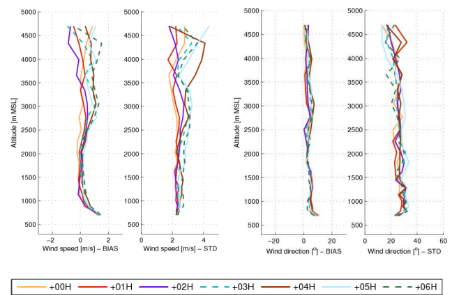
Fig. 3. Vertical profiles of wind speed bias (COSMO2-WP) and standard deviation for wind speed values between 1 and 10 \text{ms}^{-1} (left panels) and wind direction bias and standard deviation for wind speed above 3 \text{ms}^{-1} (right panels), for the first 6 forecast hours, Kleindoettingen, 1 August 2008–31 October 2008.
