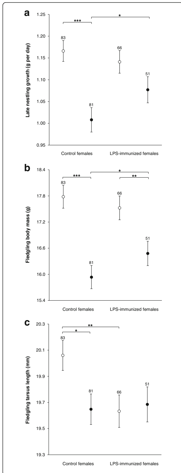
Fig. 2 Re-transformed late nestling growth ( a ), fledgling body mass ( b ) and tarsus length ( c ) in relation to maternal immunization (control vs. LPS-immunized females) and brood size manipulation (control vs. enlarged broods). Least square mean \pm SE derived from final models are shown. Open circles denote control broods, whereas filled circles denote enlarged broods. Sample sizes are noted above bars. Significant pair-wise differences are marked by * ( P < 0.05 ), ** ( P < 0.01 ) or *** ( P < 0.001 )
