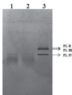
Figure 7. Analysis of the product of in vitro model of gastrointestinal digestion of M. galloprovincialis PL-proteins
