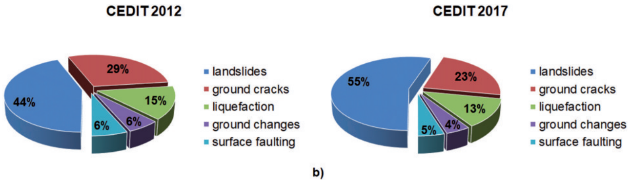
Fig. 8 - Frequency distribution of earthquake-induced ground effects distinguished for macro-categories and derived from: a) the CEDIT 2012 database and b) the CEDIT 2017 database
