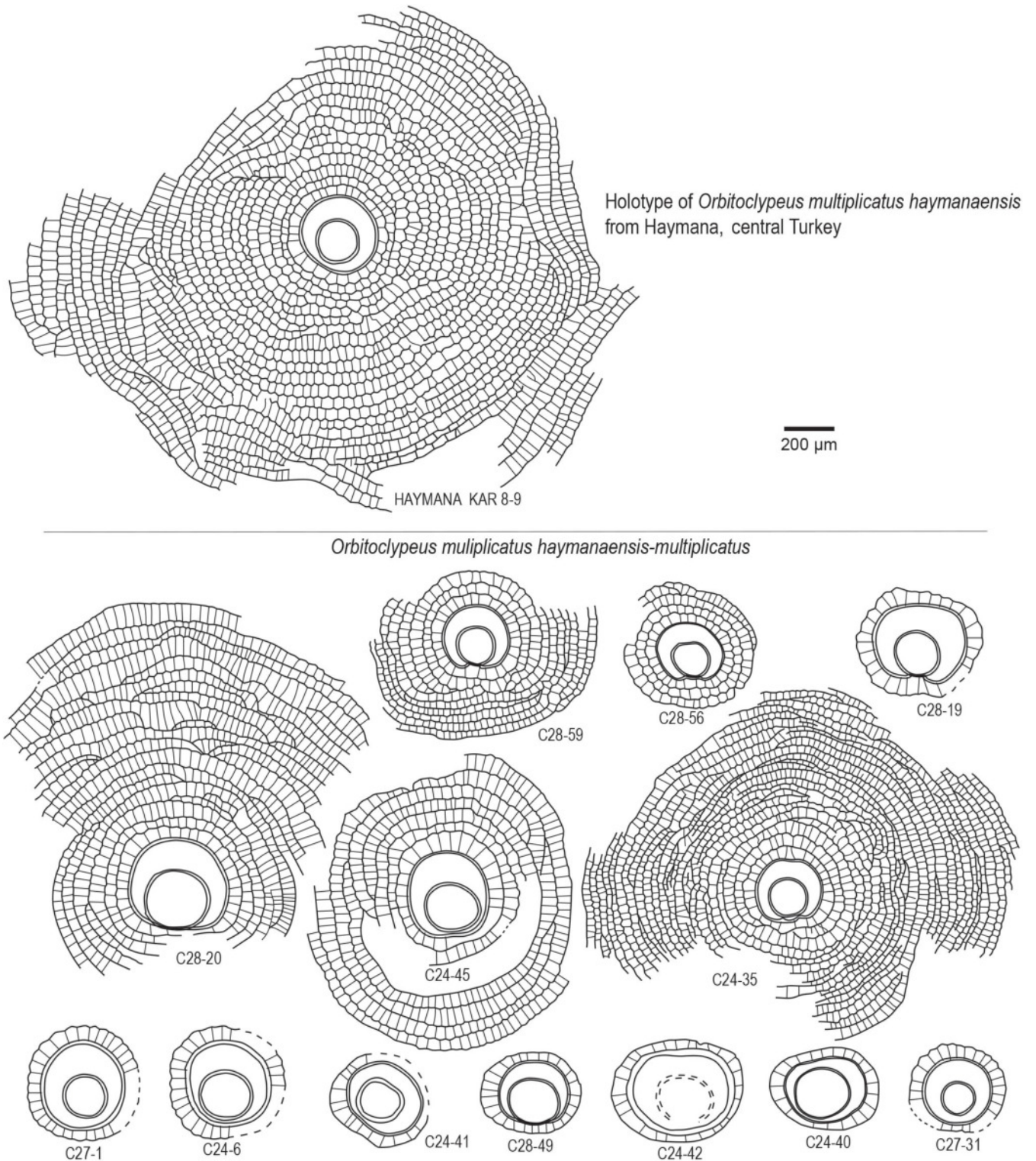
Figure 11. Embryo and equatorial chambers in Orbitoclypeus multiplicatus haymanaensis-multiplicatus . Note that the embryo is of excentrilepidine, umbilicolepidine, and trybliolepidine type, the equatorial chambers are incomplete, the distal sides of the chamberlets are arcuate to wedge shaped, and the peripheral chambers are radially elongated. The holotype of Orbitoclypeus multiplicatus haymanaensis from the Thanetian of Haymana Basin (central Turkey), sample KAR.8, is illustrated for comparison (Özcan et al., 2001).
