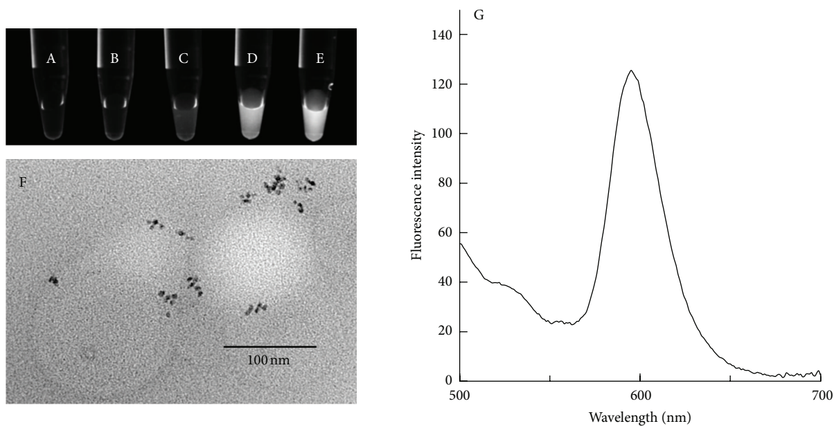
FIGURE 1: Physicochemical properties of hydrophobic (unmodified) QD-loaded SA liposomes. The lipid composition was DSPC : SA : Chol (= 8 : 0.2 : 1). Photographs of QD-loaded liposomes in phosphate buffer, (A) liposomes without QD before ultracentrifugation, (B) liposomes without QD after ultracentrifugation, and (C) 100 nM, (D) 200 nM, and (E) 400 nM QD-loaded liposomes after ultracentrifugation. All photographs were captured by placing the samples under a UV lamp. (F) TEM image of QD-loaded liposomes. The scale bar is 100 nm. (G) The fluorescence spectrum of QD-loaded liposomes was measured in phosphate buffer. Excitation was performed at 480 nm.
