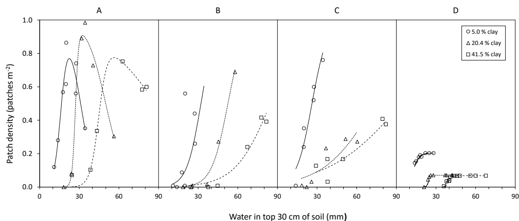
Figure 3 Examples of the relationship between availability of food types and soil water in relation to increasing clay content. Mixed grass (A); green grass (B); green forbs (C); green leaves (D). Data for green leaves from woody plants are restricted to the period from the start of leaf drop, through leaf flush, to maximum patch density.
