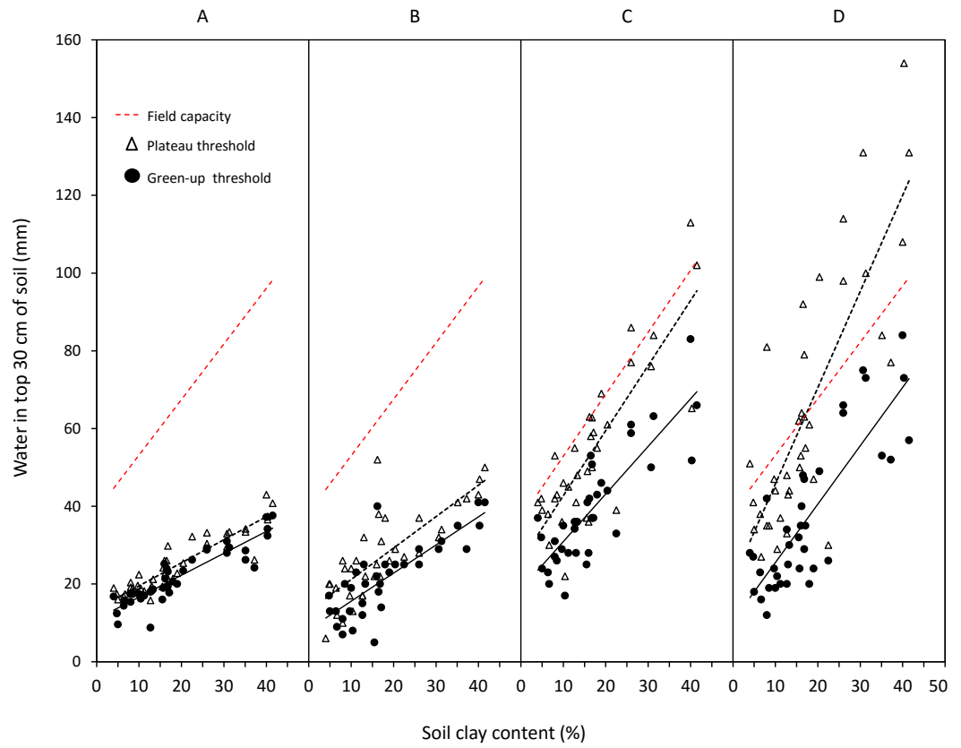
Figure 5 Linear regressions between clay content and field capacity of the 30 cm soil profile and green-up (M1) and plateau (M2) soil water thresholds for each food type. Green leaves (A); mixed grass (B); green grass (C); green forbs (D). Equations, adjusted R^2 and P values for regressions: green leaves, M_1 = 11.022 + 0.563X ( R^2 = 0.81, P < 0.001 ), M_2 = 12.645 + 0.663X ( R^2 = 0.87, P < 0.001 ); mixed grass, M_1 = 8.346 + 0.724X ( R^2 = 0.64, P < 0.001 ), M_2 = 13.423 + 0.774X ( R^2 = 0.54, P < 0.001 ); green grass, M_1 = 18.671 + 1.225X ( R^2 = 0.69, P < 0.001 ), M_2 = 26.22 + 1.673X ( R^2 = 0.70, P < 0.001 ); green forbs, M_1 = 10.52 + 1.502X ( R^2 = 0.68, P < 0.001 ), M_2 = 18.493 + 2.63X ( R^2 = 0.68, P < 0.001 ).
