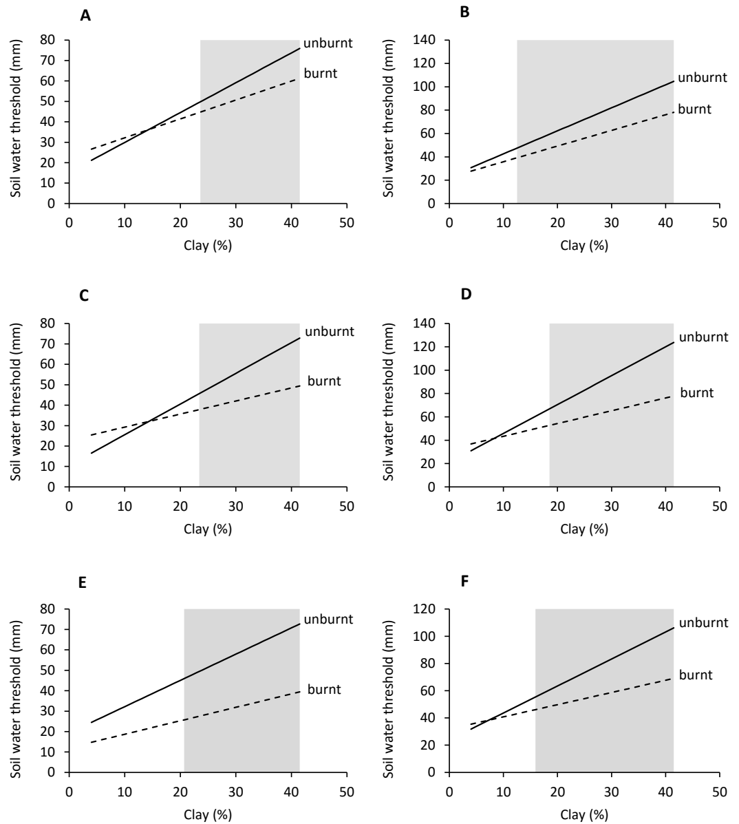
Figure 9 Effect of a significant interaction between soil clay content and fire (> 5 months previously) on soil water thresholds for green grass, green forbs and mixed grass. Green grass M_1 (A); green grass M_2 (B); green forbs M_1 (C); green forbs M_2 (D); mixed grass M_3 (E); mixed grass M_4 (F). Regions of significant ( P < 0.05 ) difference between burnt and unburnt areas are shaded grey.
