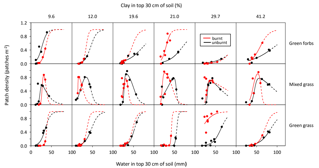
Figure 10 Examples of the effect of fire (>5 months previously) on the patch density—soil water relationship for herbaceous forage types along a gradient of increasing clay content.
