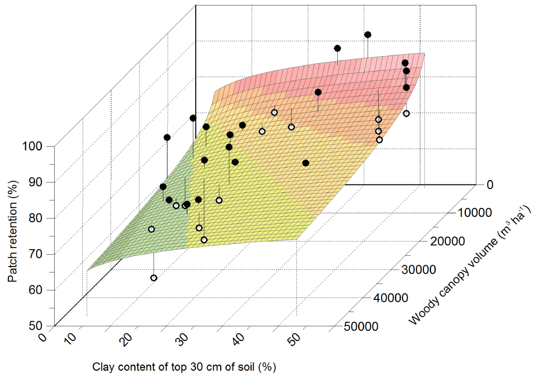
Figure 11 Influence of soil clay content and woody canopy volume on retention of green leaf patches. Y = a * (X1/X2)^b , where Y = patch retention, X1 = soil clay content, X2 = woody canopy volume, and a and b are constants.
