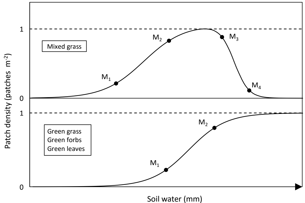
Figure 1 Sigmoidal curves representing the relationship between availability and soil water for the forage types. M_1 , threshold between lag and exponential phases (green-up); M_2 , threshold between exponential and plateau phases (plateau); M_3 , threshold between plateau and exponential phases of the decline in mixed grass patches and M_4 , threshold between exponential and lag phases of the decline in mixed grass patches.
