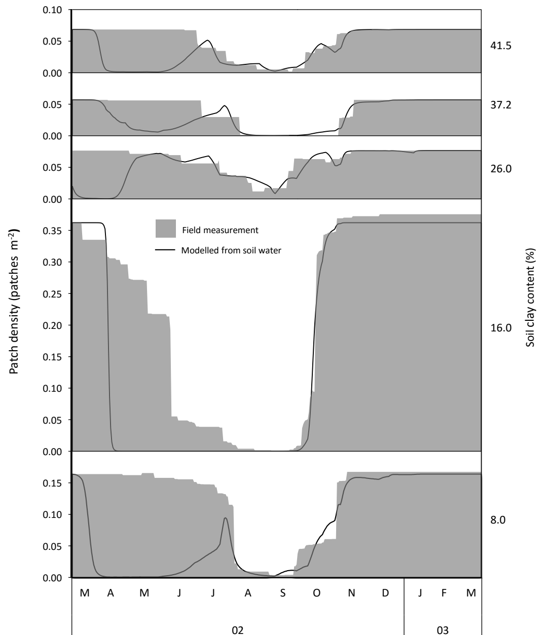
Figure 4 Examples of temporal estimates of availability of woody green leaf available to adult bull elephants from field measurements and modelling along a gradient of increasing soil clay content. Measured and modelled estimates corresponded well except for the period before leaf drop.
