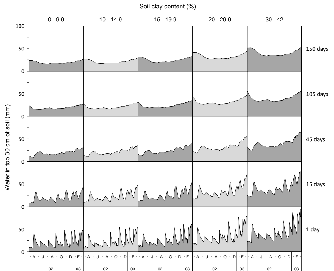
Figure 2 Effect of soil clay content and lag period on the temporal pattern of soil water.
