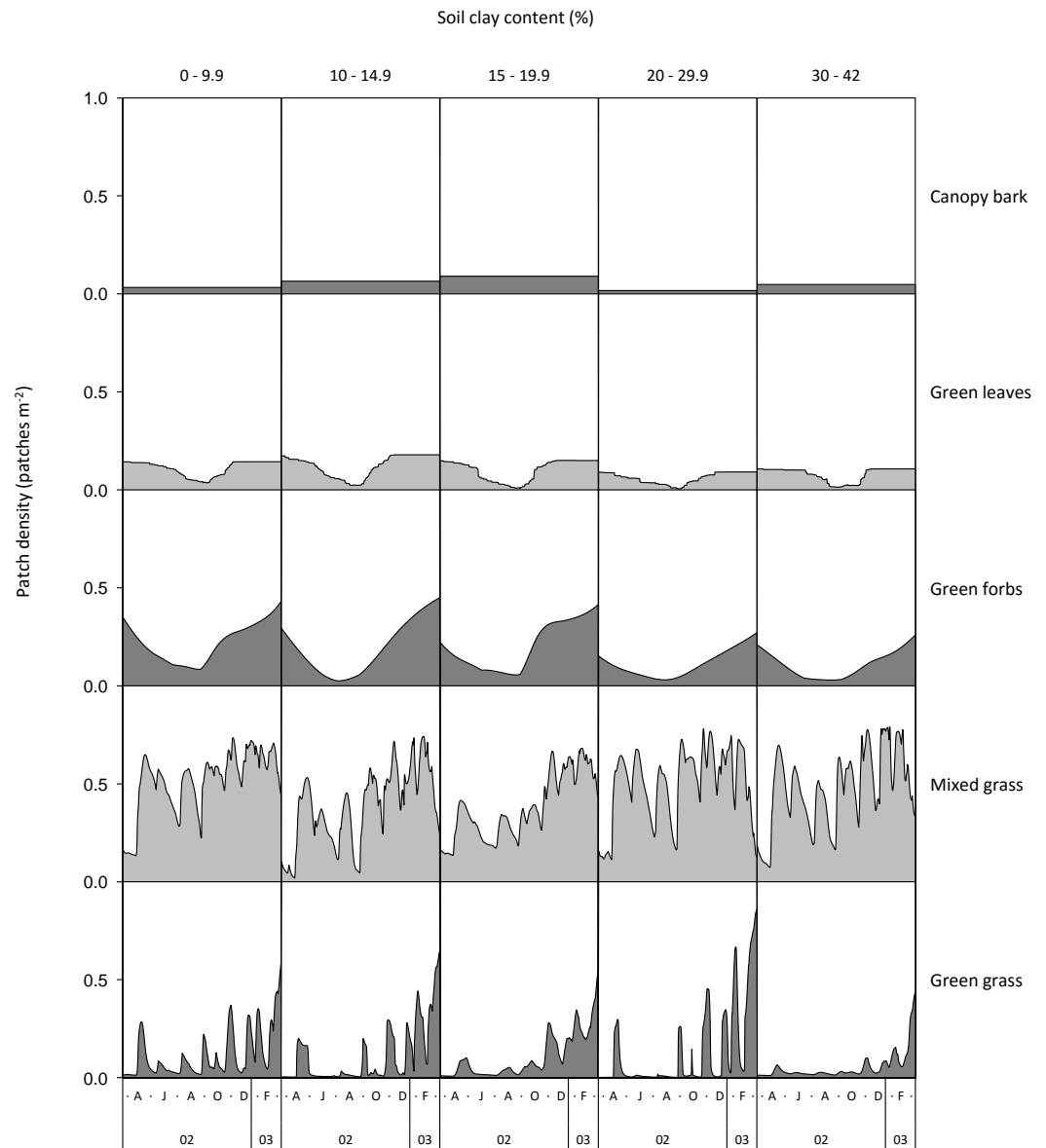
Figure 8 Temporal availability of forage types along a gradient of increasing clay content. Data for woody green leaves are for adult bulls. Availability of woody green leaf was slightly lower for cows, but otherwise followed the same pattern.
