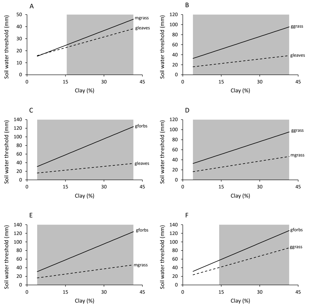
Figure 7 Effect of soil clay content and food type on plateau (M2) soil water thresholds. Regions of significant ( P < 0.05 ) differences between green leaves and mixed grass (A), green leaves and green grass (B), green leaves and green forbs (C), mixed grass and green grass (D), mixed grass and green forbs (E), and green grass and green forbs (F) are shaded grey.
