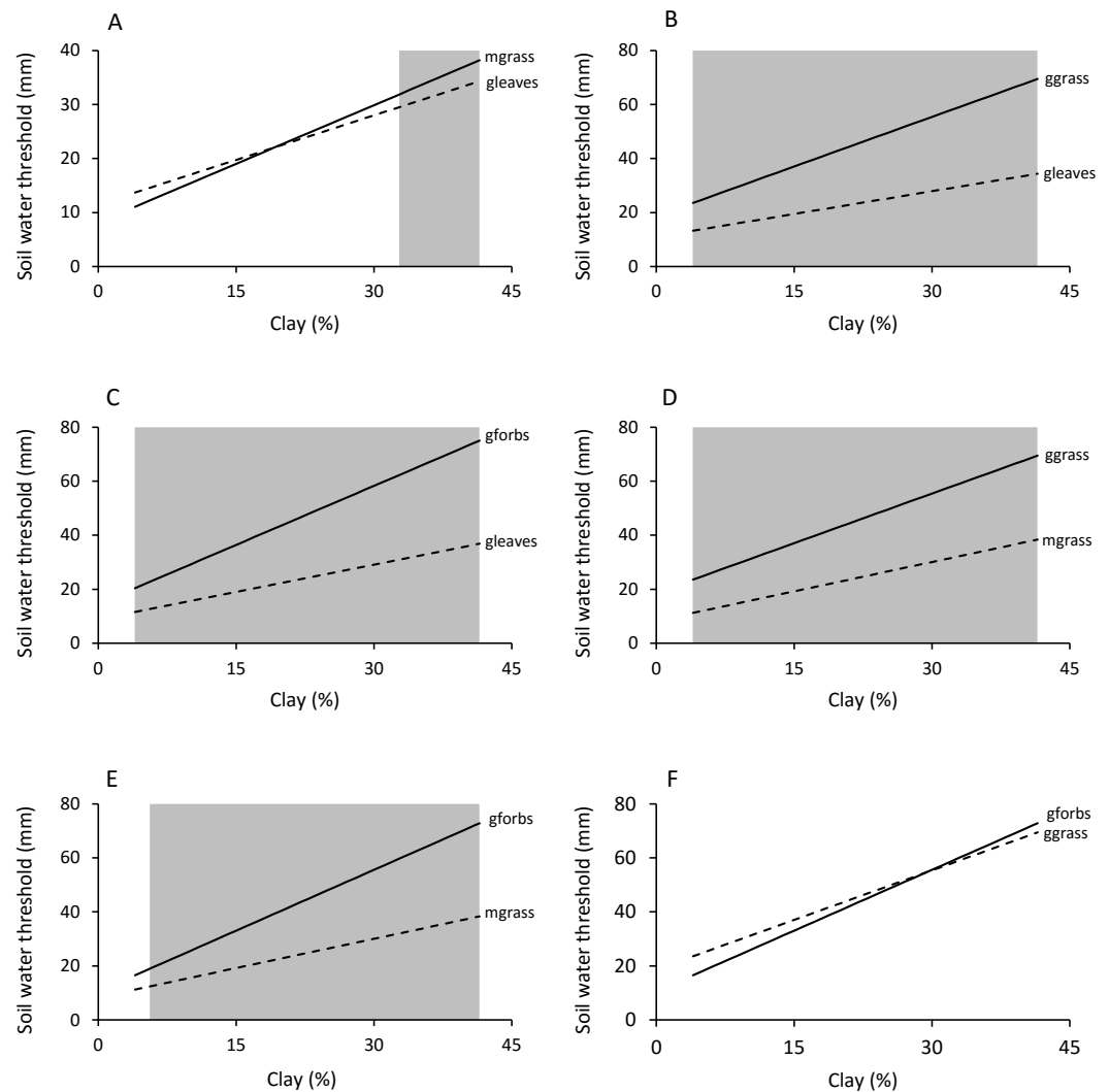
Figure 6 Effect of soil clay content and food type on green-up (M1) soil water thresholds. Regions of significant ( P < 0.05 ) differences between green leaves and mixed grass (A), green leaves and green grass (B), green leaves and green forbs (C), mixed grass and green grass (D), mixed grass and green forbs (E), and green grass and green forbs (F) are shaded grey.
