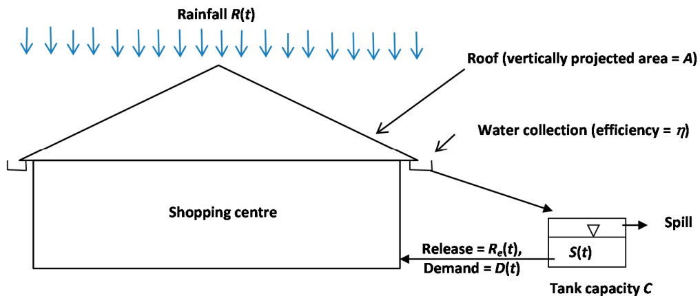
Figure 3. Rainwater harvesting system simulation components.
