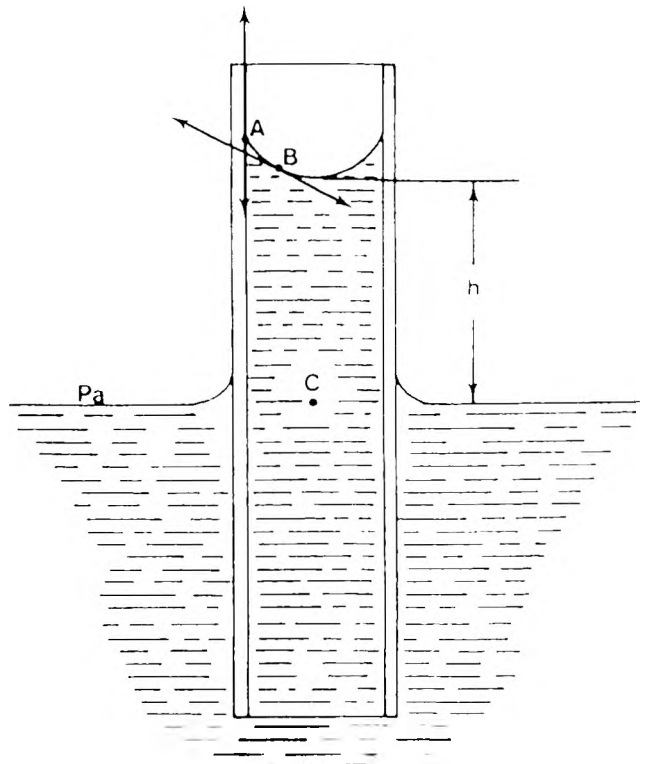
Fig. 17. Fluid rise in a capillary tube.
