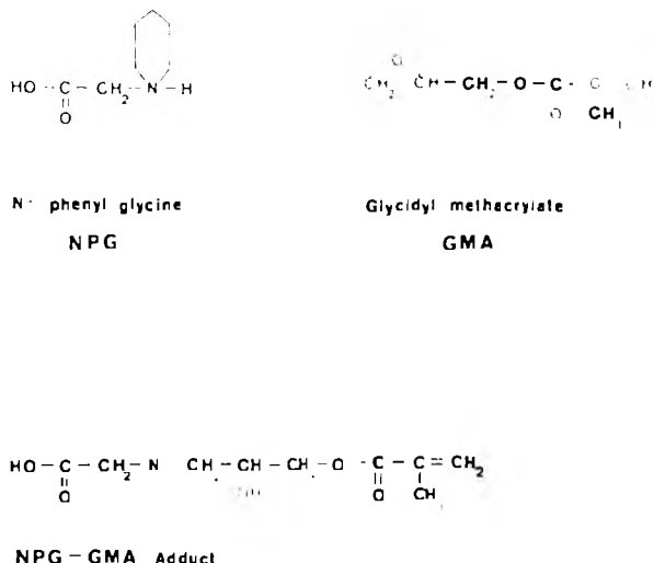
Fig. 11. Surface-active comonomer. NPG-GMA adduct. (N-(2-hydroxy-3-methacryloxypropyl)-N phenylglycine).
