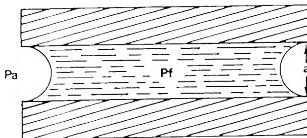
Fig. 16. Fluid film between two circular flat plates. The film thickness is a.
