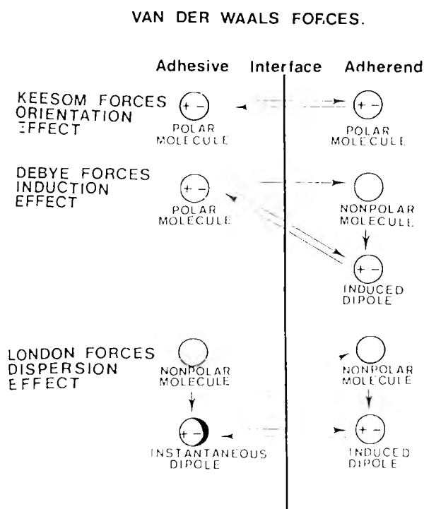
Fig. 6. Diagrammatic presentation of Van der Waals attractive forces.
