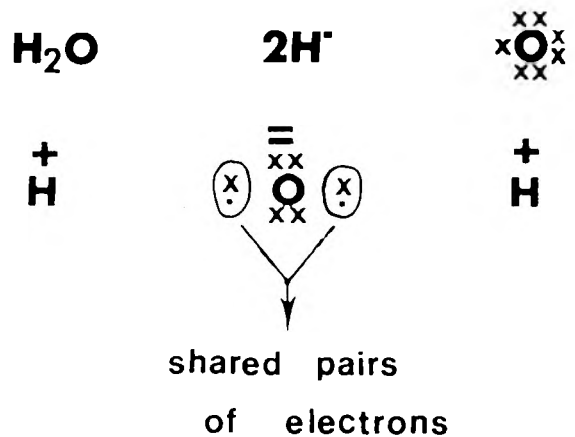
Fig. 4. Polar covalent bonds in the water molecule.
