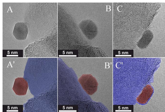
Figure 3. TEM images of Au/ \text{TiO}_2 (A) before CO oxidation, (B) after oxidation in \text{O}_2 at 0.3 mbar and room temperature and (C) CO oxidation ( \text{CO}:\text{O}_2=1:2 ) at 0.3 mbar and 100 \text{ }^\circ\text{C} . At bottom panel the images were colorized in order to highlight the differences between \text{TiO}_2 support (blue) and Au NP (red).
