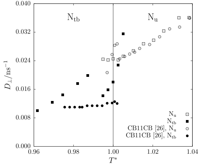
Figure 10. Dependence of the perpendicular component of the rotational diffusion tensor, D_{\perp} , on the reduced temperature, T^* \equiv T/T_{N_{tb}-N_u} , in the N_u phase (open squares) and in the N_{tb} phase (solid squares) compared to the values obtained for the related LC CB11CB [26] (open and solid circles). The vertical line indicates the approximate transition temperature observed, which is about 4 K below the transition observed by Tripathi et al. [31] for pure CB9CB. In the N_u phase, values for the CB9CB LC (open squares) are essentially identical to those for the CB11CB LC (open circles). Across the biphasic region, centred on the transition, the reorientational dynamics of the N_{tb} phase (solid symbols) is slower than that of the N_u phase (open symbols). In the N_{tb} phase, the reorientational dynamics of both LCs has values of the same order of magnitude and shows a further, almost linear decrease with the temperature (see text for details).
