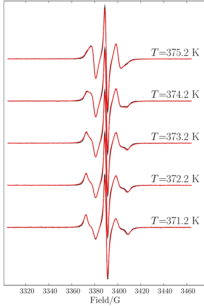
Figure 6. EPR spectra (black line) in the biphasic region of CB9CB, across the N_{tb} - N_u transition, and global fit (red line) to a model formed by two spectral contributions: one for the N_u phase, calculated according to the uniaxial nematic monodomain model, the other for the N_{tb} phase, calculated according to the distributed tilt (DT) model, presented earlier [26] (see text for details).
