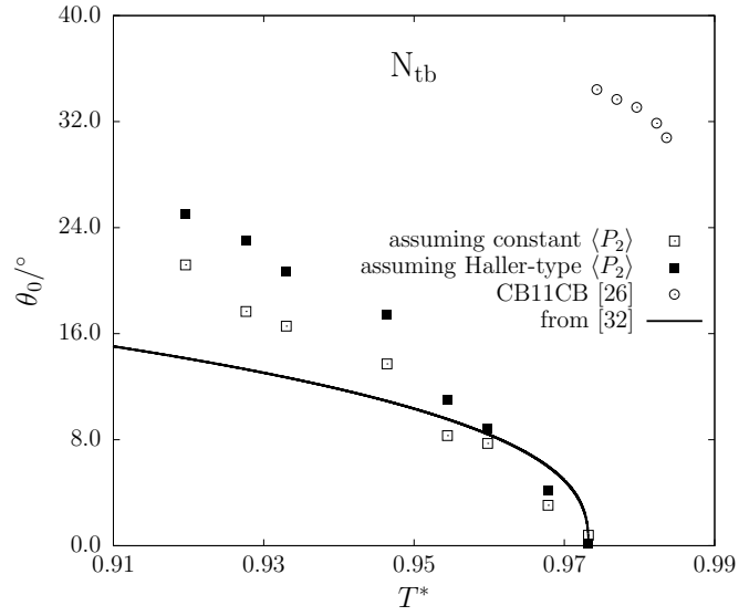
Figure 11. Dependence of the tilt angle, \theta_0 , on the reduced temperature, T^* \equiv T/T_{N_{tb}-N_u} . The values were recovered from fits of the spectra recorded in the N_{tb} phase, below the biphasic region, by adopting two different globalization schemes (open and solid squares) and are compared to the values obtained for the related LC CB11CB [26] (open circles) and to the Haller-type \theta_0 temperature dependence obtained for the CB9CB LC by Robles-Hernández et al. [32] (solid line) with the zero of the Haller function shifted at 363.2 K, which corresponds to the first temperature considered in the N_{tb} phase, below the biphasic region. In the first globalization scheme (open squares), the local \langle P_2 \rangle was assumed to be constant across the N_{tb} phase, below the biphasic region. In the second (solid squares), the local \langle P_2 \rangle had the empirical Haller-type temperature dependence of equation 7 ( T_{NI} = 389.2 K, \langle P_2 \rangle_0 = 0.97 , \beta = 0.21 ), shown as a solid line in Figure 9 (see text for details).
