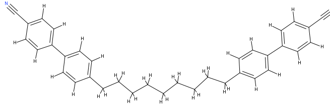
Figure 1. Molecular structure of CB9CB.
