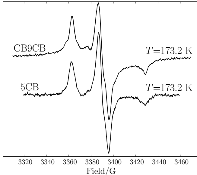
Figure 3. Rigid-limit spectrum of CB9CB compared with a rigid-limit spectrum of 5CB. Both spectra were recorded in the bulk at 173.2 K.
