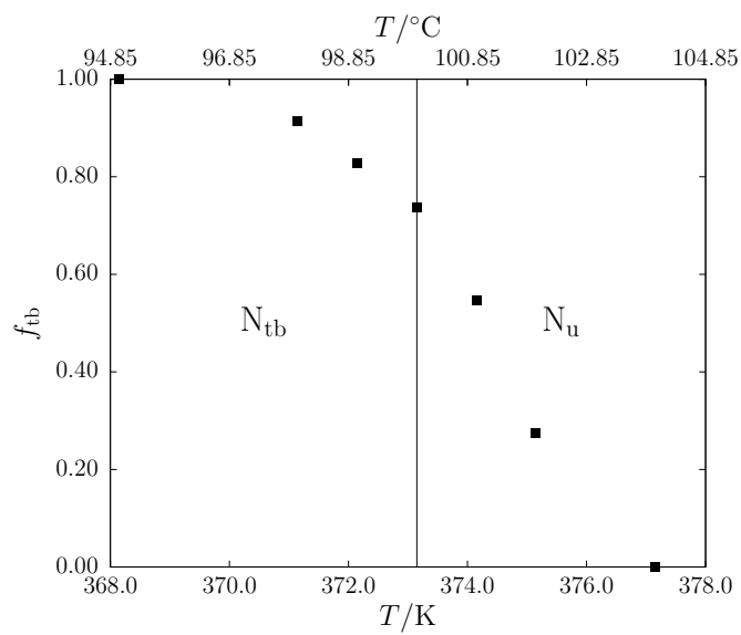
Figure 7. Temperature dependence of the fractional contribution of the spectral component due to the N_{tb} phase, f_{tb} , across the biphasic region of CB9CB, obtained from the global fit presented in Figure 6 (see text for details).
