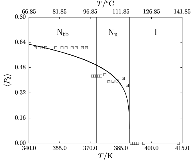
Figure 9. Temperature dependence of the local orientational order parameter, \langle P_2 \rangle , across the full temperature range studied (open squares), compared with values calculated with the Haller function of equation 7 ( T_{NI} = 389.2 K, \langle P_2 \rangle_0 = 0.97 , \beta = 0.21 , solid line, see text for details). Vertical lines indicate the approximate transition temperatures observed, that are about 4 K below the transitions observed by Tripathi et al. [31] for pure CB9CB. In the biphasic region (series of five points centred on the N_{tb} - N_u transition), \langle P_2 \rangle best-fit value was 0.43 for the N_u phase (data points shown) and 0.39 for the N_{tb} phase (not shown).
