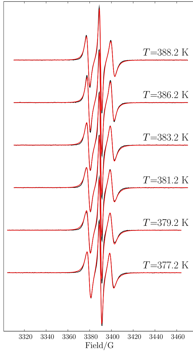
Figure 5. EPR spectra in the N_u phase of CB9CB (black line) and fit to the uniaxial nematic monodomain model (red line).
