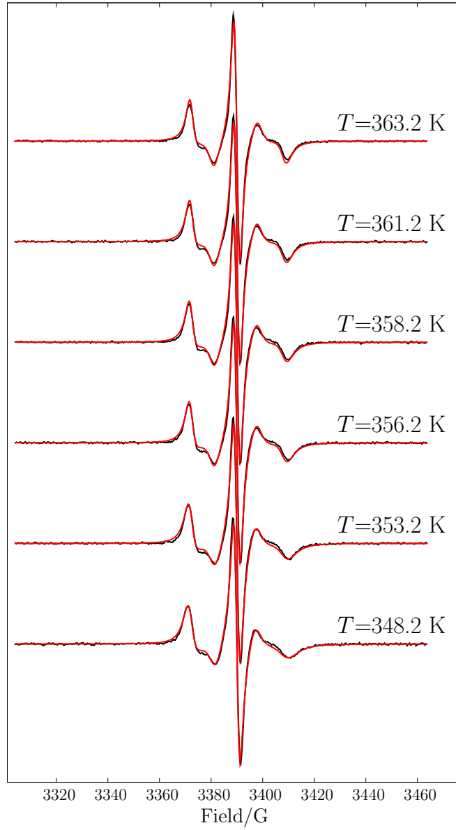
Figure 8. EPR spectra in the N_{tb} phase (black line) and fit to the distributed-tilt (DT) model (red line). Local \langle P_2 \rangle was assumed to be independent of the temperature and treated as a global parameter. Best-fit value was 0.61. Best-fit values of the tilt angle, \theta_0 , are presented in Figure 11 (open squares, see text for details).
