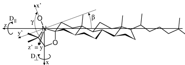
Figure 2. Molecular structure of the CSL spin probe together with the chosen ordering ( x, y, z , solid line) and magnetic ( x', y', z' , dashed line) molecular frames, the Euler angles, \beta and \gamma , between the molecular frames and the principal components, D_{\perp} (reorientation of the molecular long axis) and D_{\parallel} (rotation around the molecular long axis), of the rotational diffusion tensor.
