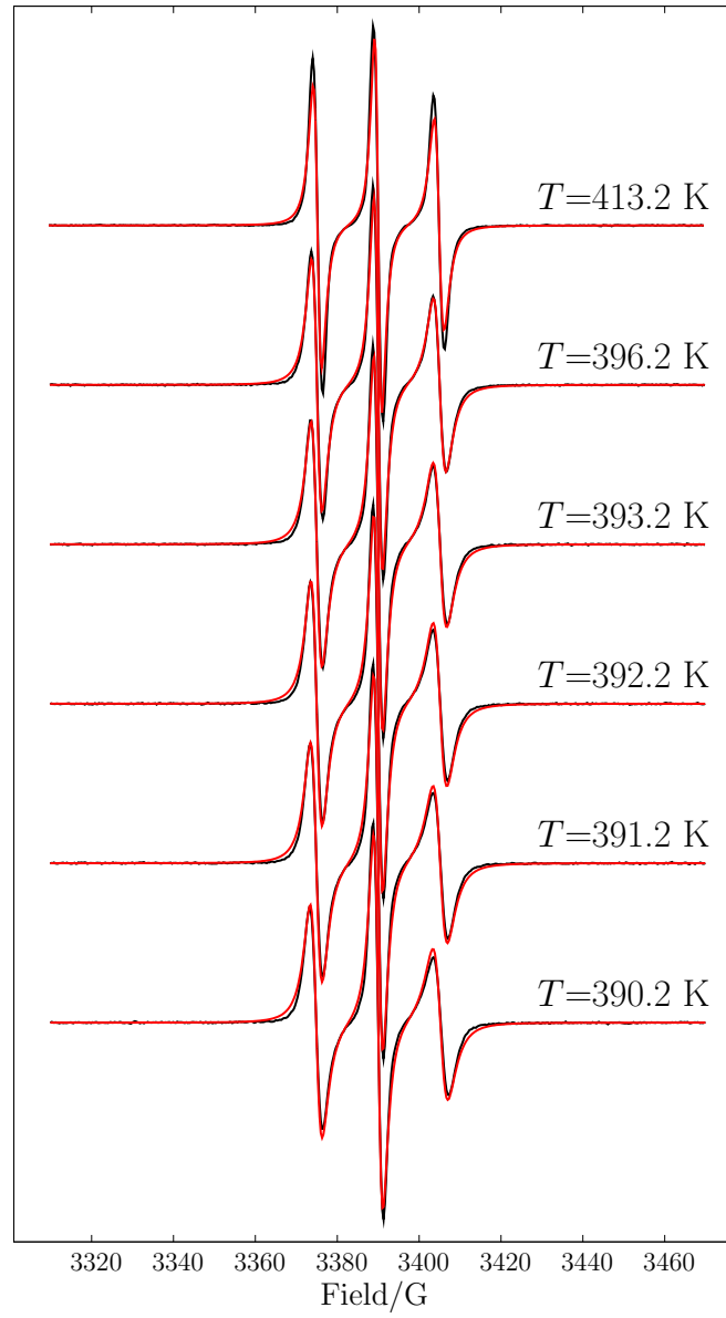
Figure 4. EPR spectra in the I phase of CB9CB (black line) and fit to the isotropic model (red line).
