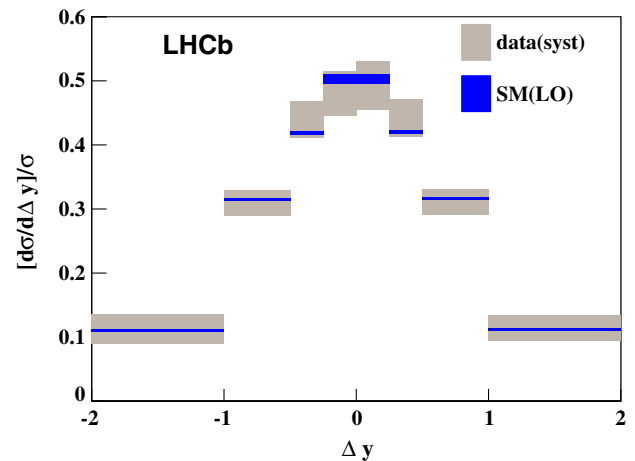
FIG. 4 (color online). Corrected \Delta y distribution for all selected events. The statistical uncertainties are negligible. The systematic uncertainties are highly correlated from bin to bin and largely cancel in the determination of A_C^{b\bar{b}} . The LO SM prediction obtained from PYTHIA [36,37] is also shown.
