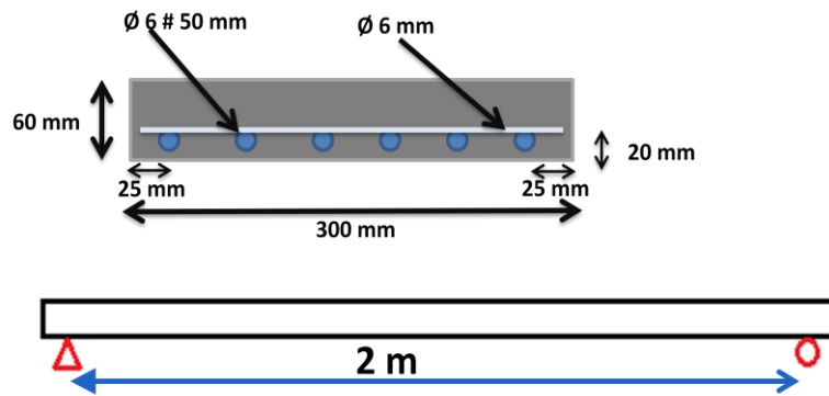
Fig.1: RC slab details.
