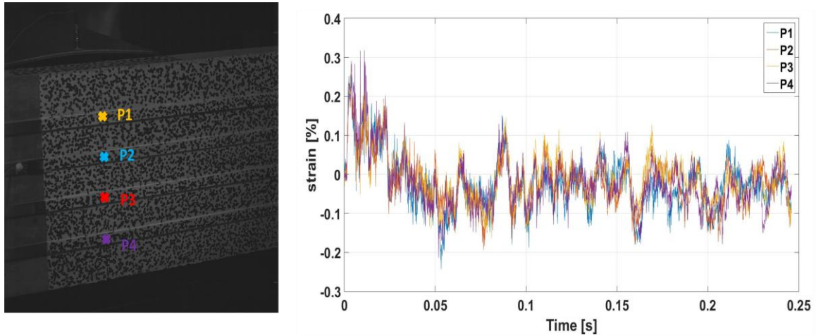
Fig.9: Strain distribution in the CFRP strips for test 4.
