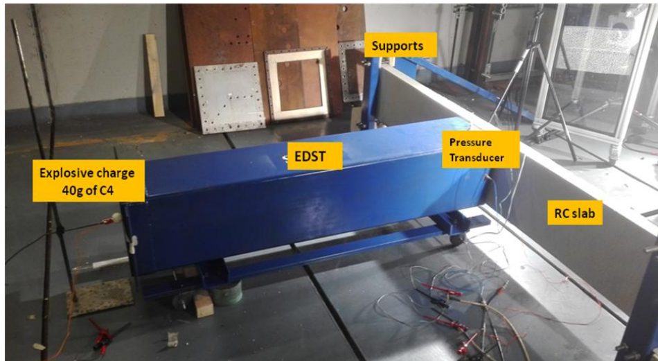
Fig.3: Experimental setup for blast tests.
