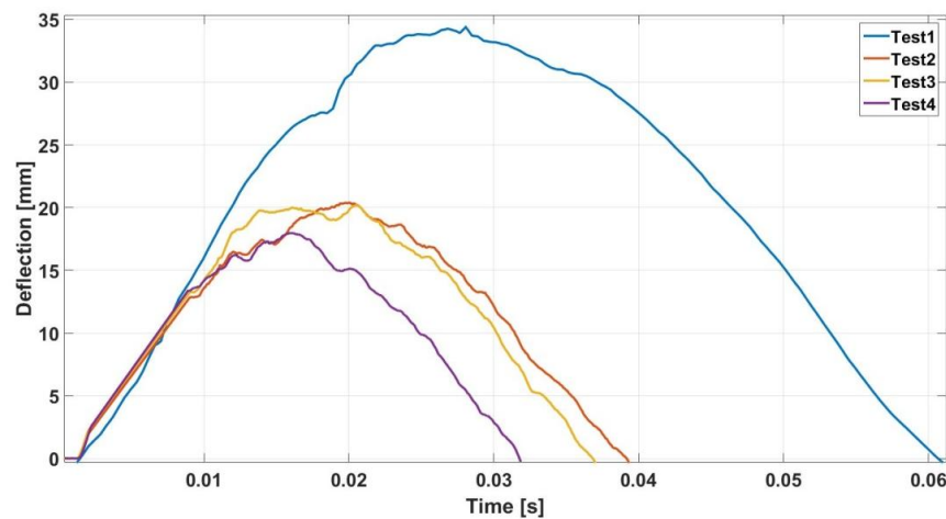
Fig.5: Deflection time histories for experimental tests with DIC measurement.
