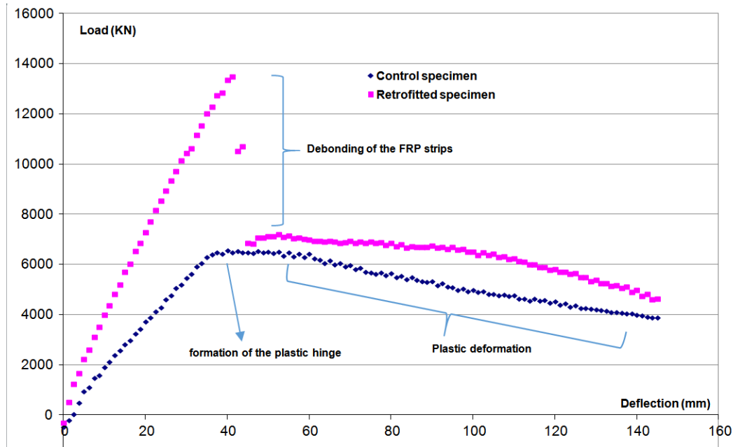
Fig.11: Load-deflection diagram
