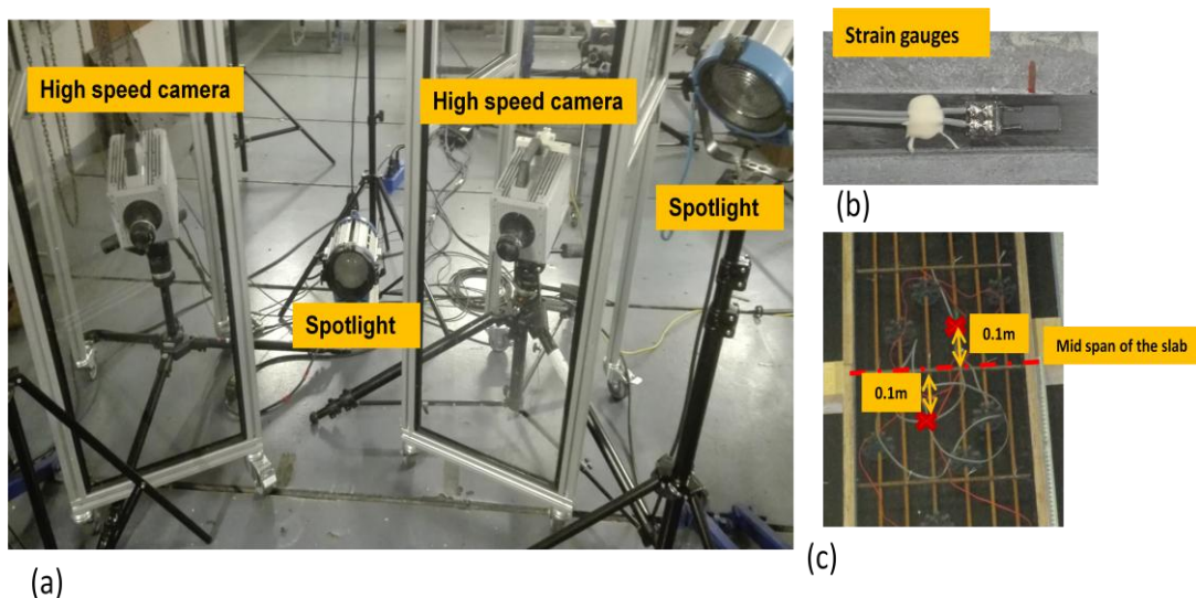
Fig.4: (a) Stereo vision setup of two high speed camera for DIC measurements; (b) strain gauge bonded on CFRP strip; (c) strain gauges glued on steel rebars before casting the concrete.
