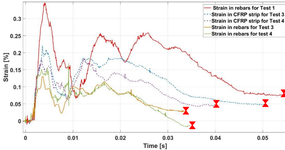
Fig.7: Evolution of the strain in the steel rebars and in CFRP strips during the inbound phase (X impact with the tube)
