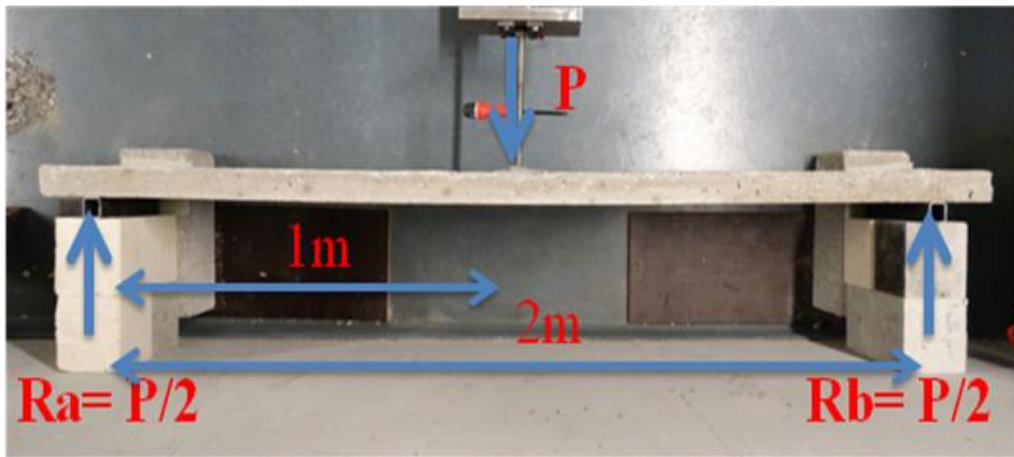
Fig.10: Experimental set-up of static tests
