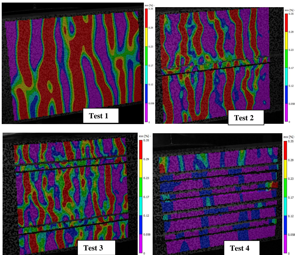
Fig.8: Strain distribution on the concrete and the FRP strips using DIC measurement .
