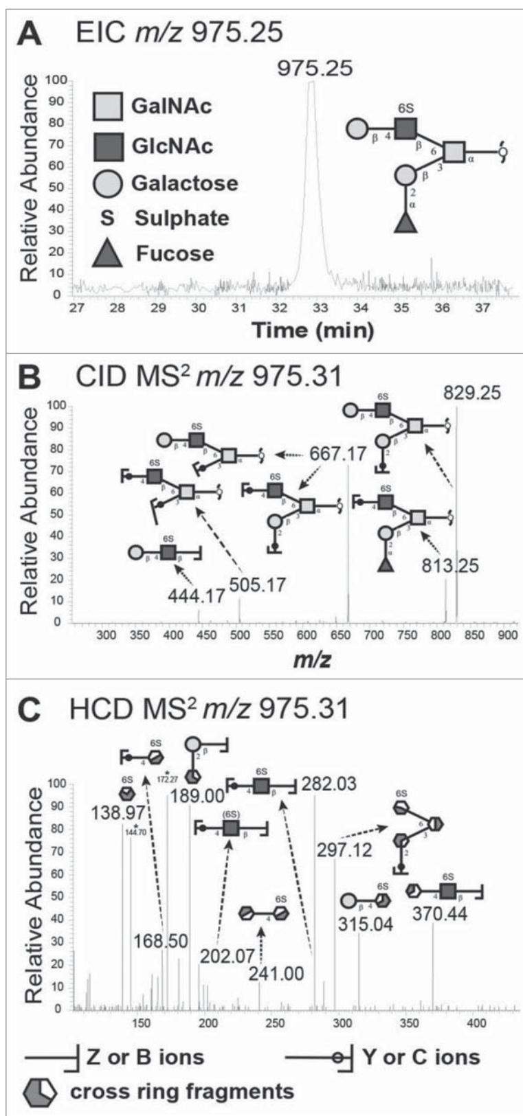
Figure 8. Identification of the m/z 975.25 structure (Gal \beta 4(6S)GlcNAc \beta 6(Fuc \alpha 2Gal \beta 3)GalNAc \alpha 1) from porcine gastric mucin O -glycans by LC-MS/MS. A. Extracted ion chromatogram (EIC) of m/z 975.25 [M-H] - . B. Collision-induced dissociation (CID)-based MS/MS fragmentation spectra with annotated fragments. C. Higher-energy collisional dissociation (HCD)-based MS/MS low mass region ( m/z 110–390) showing fragments specific for blood group H on C3 arm and a type 2 LacNAc on C6 with 6-linked sulfate on GlcNAc. * denotes background ions. The Consortium for Functional Glycomics cartoons were used to represent O -linked glycan structures.
