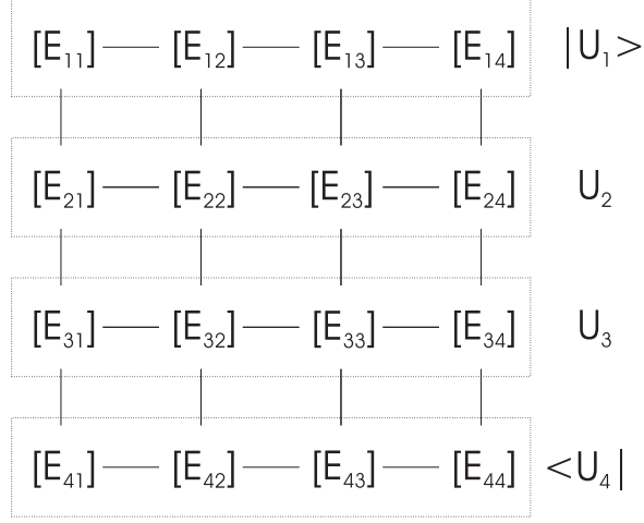
Figure 18: Structure of the contractions in \langle \Psi_A | \Psi_A \rangle . In this scheme, the first and last rows can be interpreted as MPS |U_1\rangle and \langle U_4| and the rows in between as MPO U_2 and U_3 . The contraction of all tensors is then equal to \langle U_4 | U_3 U_2 | U_1 \rangle .
