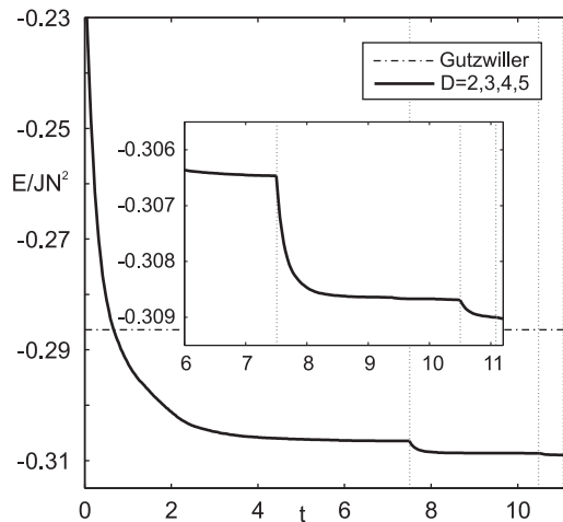
Figure 20: (taken from [75]) Energy as a function of time for the imaginary time-evolution of the system of hard-core bosons on a 11 \times 11 -lattice. The evolutions are performed sequentially with PEPS of virtual dimension D = 2 , D = 3 , D = 4 and D = 5 . The times at which D is increased are indicated by vertical lines. For comparison, the energy of the optimal Gutzwiller ansatz is included.
