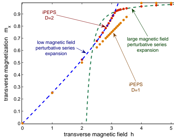
Figure 23: (taken from [56]) Magnetization m_x(h) in the ground state |\Psi_h\rangle of the two-dimensional quantum Ising model with transverse magnetic field. A trivial iPEPS (inner dimension D = 1 ) produces a magnetization that grows essentially linearly with the magnetic field until it saturates. Instead, the simplest non-trivial iPEPS (inner dimension D = 2 ) produces a magnetization curve that overlaps with the results of series expansions for both small and large magnetic fields. [ D = 3 leads to results that could hardly be distinguished from those for D = 2 in this figure]. Notice that around h \approx 3.1 the derivative of the magnetization m_x(h) changes suddenly.
