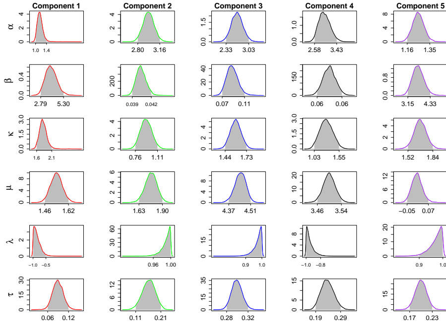
Fig. 9: Posterior densities of the parameters for best Abe-Ley mixture model for EV arrival
