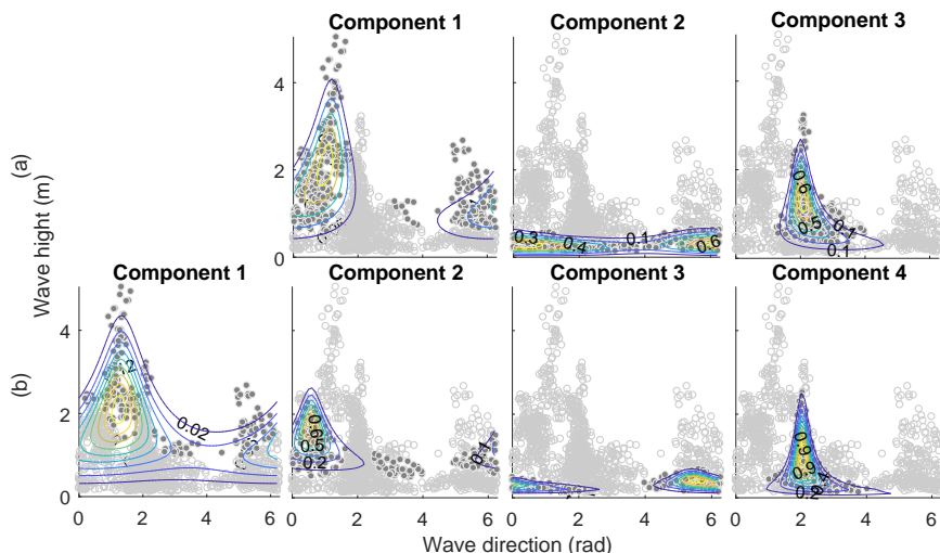
Fig. 7: Component-wise densities for (a) Abe-Ley mixture model estimated by [11] and (b) Abe-Ley mixture model estimated by our proposed approach.
