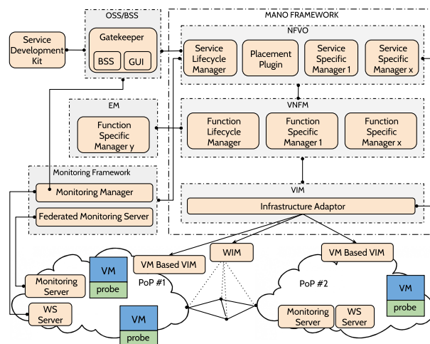
Fig. 1: SONATA ETSI conform Architecture
