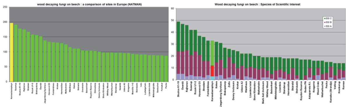
Fig 2 : figure on total species richness and Species of Scientific Interest (SSI) for the Nat-Man sites. Highlighted is the sampling site at Sonian forest.
