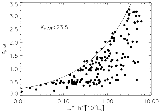
FIG. 7.—The L_V - z diagram for the objects selected in our sample with K_{s,AB} < 23.5 . The tracks represent the values of L_V^{\text{rest}} for Scd template spectra (see Fig. 11c in Rudnick et al. 2001) normalized at each redshift to K_{s,AB} = 23.5 .
