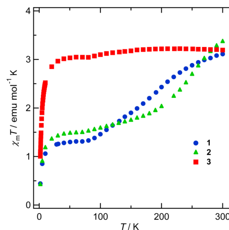
Fig. 6. Magnetic properties of 1 (●), 2 (▲), and 3 (◻).
