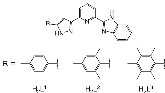
Scheme 1. Three asymmetric tridentate ligands L^1 - L^3 .
