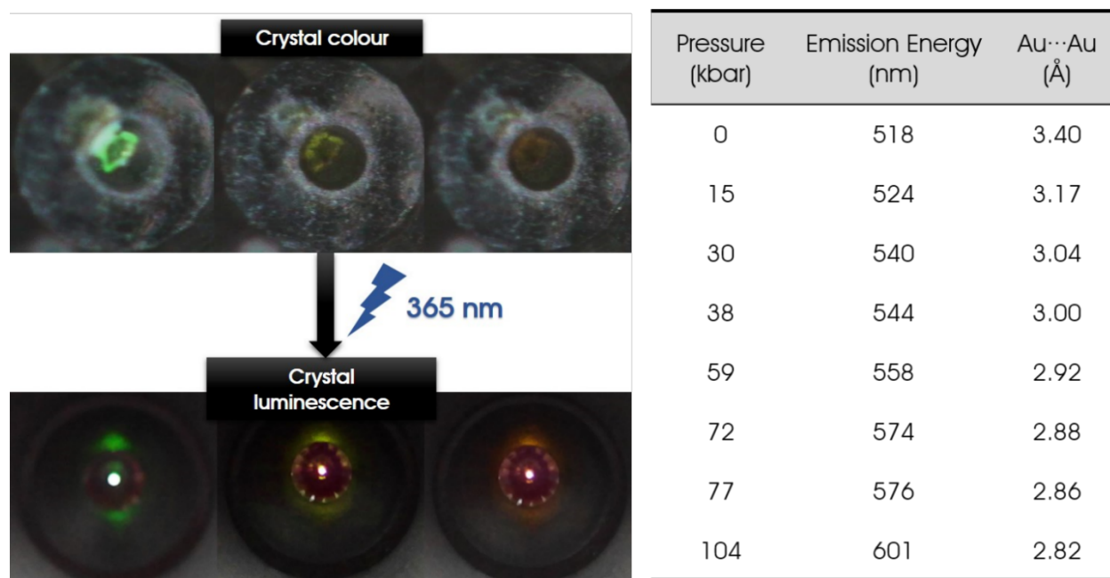
Figure 2. Left: (top) Crystal colour at ambient pressure (green), between 34.3 and 48.7 kbar (yellow) and above 53.7 kbar (orange). (bottom) Crystal luminescence at 14.7 kbar (green), at
