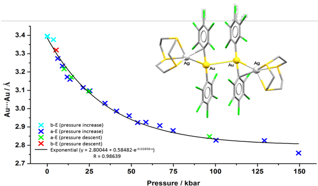
Figure 1. Molecular structure and pressure dependence of the Au...Au distance for the E - [\text{Au}(\text{C}_6\text{Cl}_6)_2\text{Ag}([\text{9}]\text{aneS}_6)]_2 .
