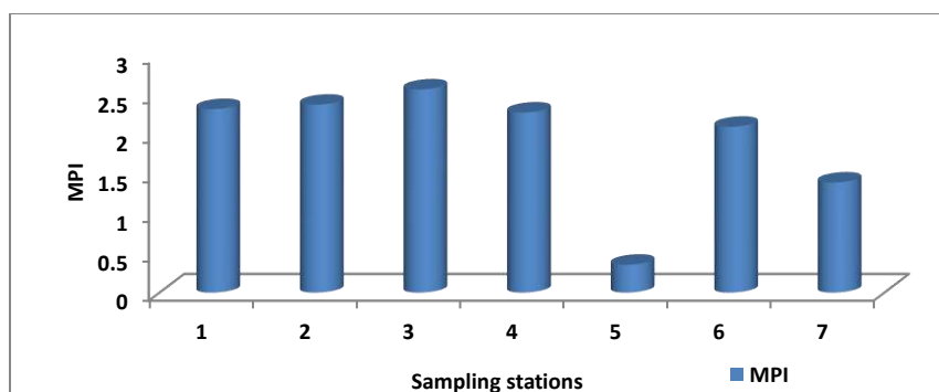
Fig. 3. Variation of metal pollution index of heavy metals in sediments from Achankovil river basin.
