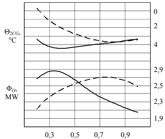
Fig. 3. Dependence of CG cooling temperature \Theta_{2CG} and the ARU cooling capacity \Phi_O on the control action related to the consumption of reflux M_R at different values of the refrigerant concentration \xi_X^{IN} at the inlet to the evaporator: — \xi_X^{IN} = 0,998 \text{ kg/kg} ; - - - \xi_X^{IN} = 0,994 \text{ kg/kg}
