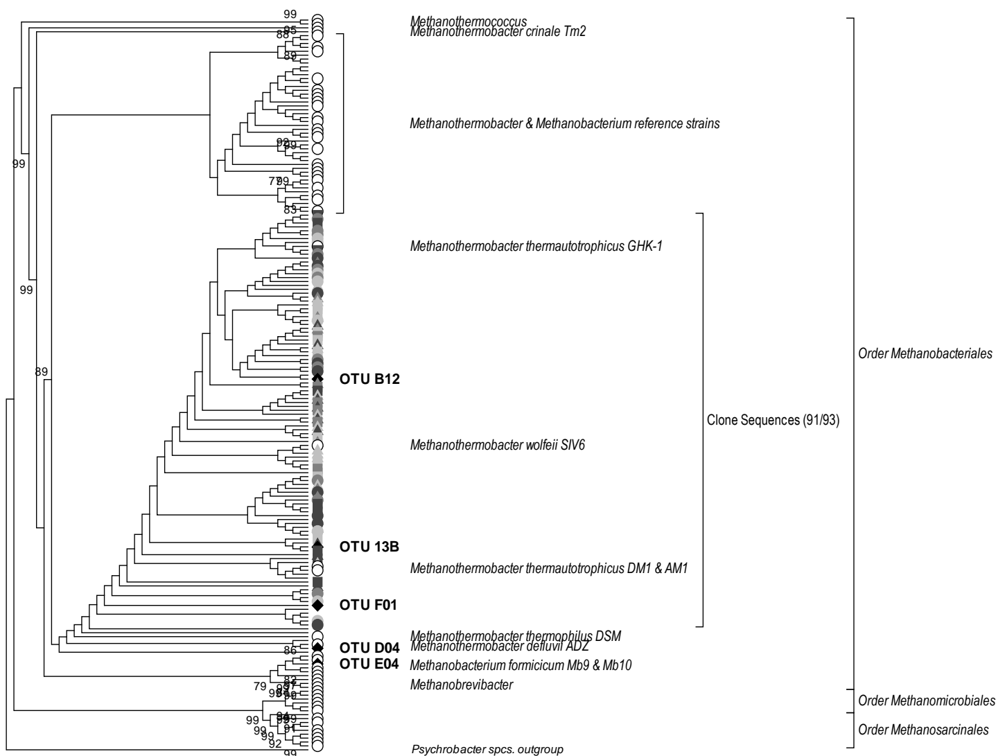
Figure 2: Consensus tree (Neighbour-Joining method with Tamura-Nei distances through 1000 iterations, showing evolutionary distances between cloned and reference sequences in this study.
