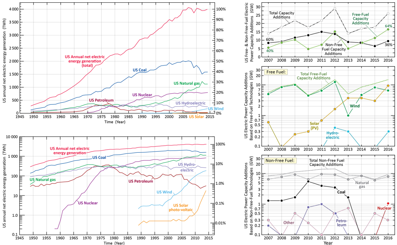
Figure 3: (Left) Historical development of the generation of electric energy in the U.S., on linear (top) and logarithmic (bottom) scales. In the US, the annual electric energy generated by wind energy is expected to exceed hydro-electric energy in a few years. (Right) Historical development of new electricity generating capacity, both total (top) and broken out by free-fuel (middle) and non-free-fuel (bottom) sources.
