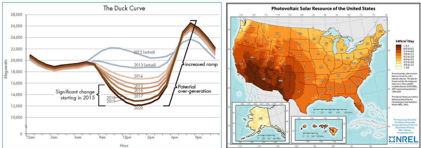
Figure 6: (a) A "duck" curve 56 illustrating the forecasted hourly mismatch in California, from midnight to midnight, between the total demand for electricity, and the anticipated supply of solar electricity, as the projected penetration of solar electricity increases from 2013 to 2020. During the mid-day hours, from 10a until 4p, the solar resource is high, so demand-minus-supply is lowest (the belly of the duck). During the early evening hours, from 6p until 8p, residential demand spikes but the solar resource is low, so demand-supply is highest (the head of the duck). During the late evening and early morning hours, from 10p until 9a, demand is low and the solar resource is also low, so demand-minus-supply is moderate (the tail of the duck). Licensed with permission from the California ISO (Independent System Operator). (b) A "heat map" of the geographic variation of the solar resource in the U.S. The regions of high solar resource (high solar electricity supply) do not generally overlap the regions of high population density (high electricity demand). The map was created by (and reproduced here courtesy of) the National Renewable Energy Laboratory for the U.S. Department of Energy.
