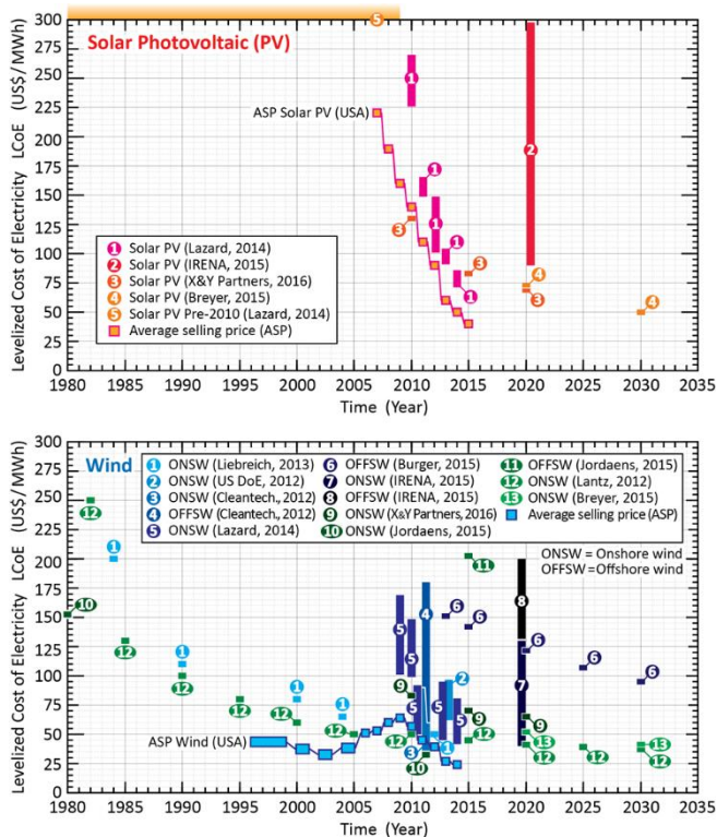
Figure 4: Levelized Costs of Electricity (LCOE), both actual and projections, for solar and wind, compiled from various sources. Average Selling Prices (ASPs) in the U.S. are also indicated; from 1980 to 2009, based on data published by Lazard (2014), the LCOE for solar photovoltaics exceeded 300 US$/MWh, as indicated by the horizontal orange bar at the top. LCOEs are beset with uncertainties that include future interest rates and payments that are part of the capital expenses (Capex). In contrast, ASPs do not include such uncertainties. Accordingly, the (estimated) LCOEs and the (precise) ASPs can be (substantially) different. Furthermore, given that the LCOE includes uncertainties, there are inevitably differences amongst the LCOE values originating from multiple literature sources. These differences are consistent with the spread of data displayed in the figure.
