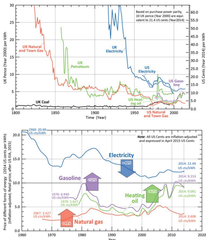
Figure 2: (a) (Top) Long-term (1800-2014) inflation-adjusted absolute UK and U.S. consumer prices per kWh of different energy currencies versus time using purchase power parity for the conversion of UK Pence to U.S. Cents. Inspection of the figure shows a general trend of a long-term decreasing cost of most of the energy currencies, including electricity. (b) (Bottom) Shorter term (1960-2014) inflation-adjusted U.S. consumer prices of different energy currencies versus time (expressed in 2015 U.S. Cents). The shorter-term price of electricity has been decreasing whereas that of other energy currencies has been increasing.
