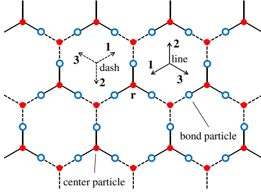
FIG. 1 (color online). The two-dimensional system composed of spin-3/2 particles. The system is a hexagonal lattice, where center particles (red round) are located on vertices, while bond particles (blue ring) are located on edges. There are two kinds of interactions between center particles and bond particles, V_{\text{line}} (line) and V_{\text{dash}} (dash line). \mathbf{r} denotes the position of a center particle, and the vectors between the center particle and its three interacting bond particles are \mathbf{1} , \mathbf{2} , \mathbf{3} respectively.
