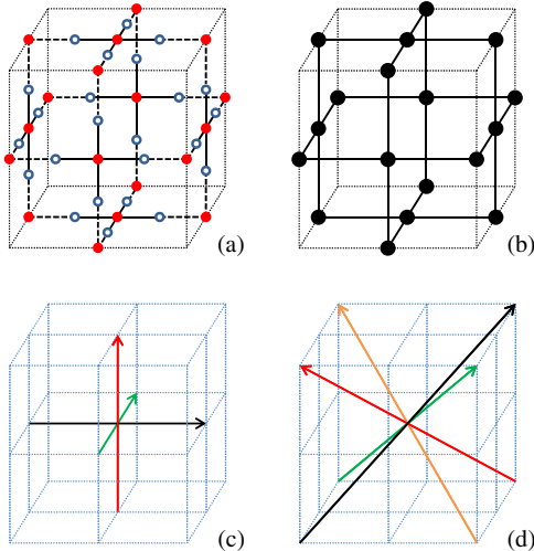
FIG. 2 (color online). The three-dimensional system. (a) The elementary cell of the system. The system is composed of spin-2 particles and spin-3/2 particles. Spin-2 particles are center particles (red round), and spin-3/2 particles are bond particles (blue ring). (b) The elementary cell of the three-dimensional topology protected cluster state, which can be prepared by single-particle operations and measurements on the ground state of the 3D system. (c) Three directions for k \leq 3 of the POVM on spin-2 particles, which are orthogonal with each other and passing face centers of a cube. (d) Four directions for k \geq 4 of the POVM on spin-2 particles, which are along body diagonals of the same cube.
