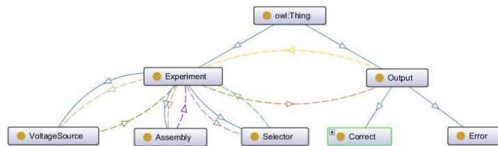
Fig. 3. Domain ontology used in the analysis of the experiments and recommendation of possible errors.
