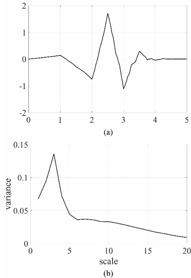
Figure 2. Wavelet filter and variance curve. (a) Wavelet function of the Daubechies-3 (db3) wavelet; (b) Variance curve of wavelet coefficients at different scales, using db3 filter.
