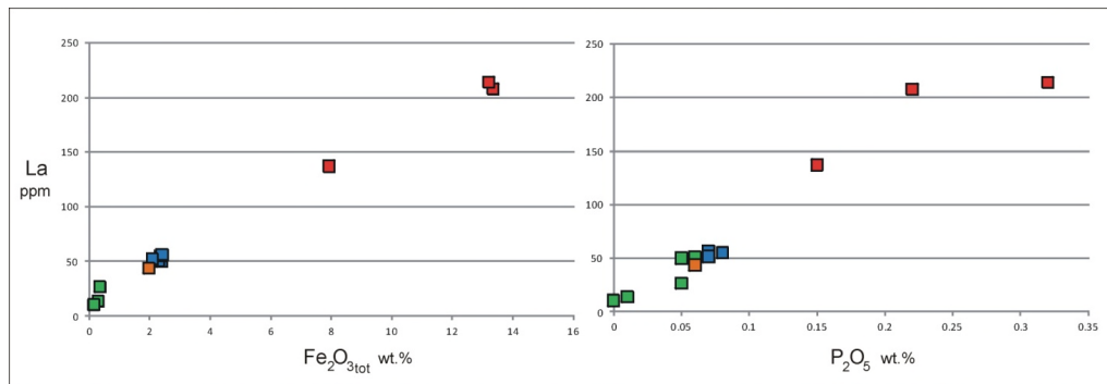
Figure 7: La- \text{Fe}_2\text{O}_3 and La- \text{P}_2\text{O}_5 correlations. La as ppm, \text{Fe}_2\text{O}_3 and \text{P}_2\text{O}_5 as wt.%. Blue: rock waste; red: treatment plant, magnetic fraction; green: treatment plant, amagnetic fraction; orange: feeding material.
