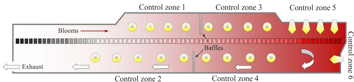
Fig. 1. Outline of the reheating furnace under steady state operation.
