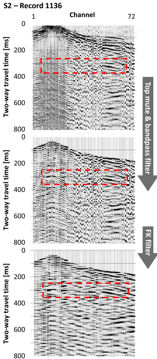
Figure 8. To eliminate noise and harmonic distortions, a bandpass filter and individual FK filters were applied to the records of each profile. The filtering in the frequency–wavenumber domain was one of the key processing steps to get interpretable seismic sections (note red box, showing the improved S/N ratio of near-surface reflectors).
