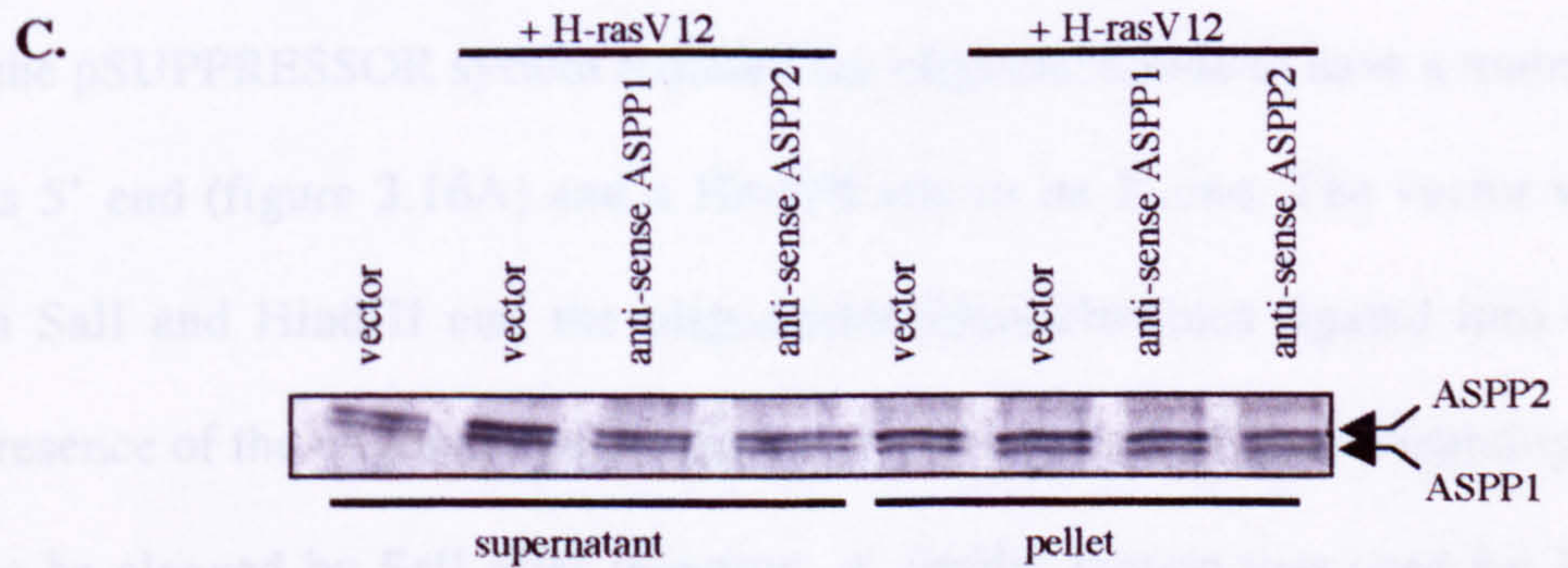
Figure 3.15 H-rasV12 and K-rasV12 activate endogenous ASPP1 and ASPP2 . (A) MCF7 cells were transfected with 6 \mu g anti-sense ASPP1 or anti-sense ASPP2 , in the presence or absence of 1.5 \mu g of H-rasV12 or K-rasV12 . All cells were co-transfected with bax-luciferase reporter. The cells were harvested and lysed with the luciferase lysis buffer (Promega) and a luciferase assay carried out. (B) A similar experiment to A was performed in U2OS cells with PIG3-luciferase reporter. The lysate was used for Western blotting and the presence of transfected H-rasV12 and K-rasV12 was detected with the HA antibody. (C) Lysates 1 and 4-6 from B were taken and the supernatant separated from the pellet. The pellet was further resuspended in 1x RIPA buffer. An equal amount of protein was loaded onto a 8% SDS-PAGE gel and western blotting was performed to detect ASPP1 and ASPP2 with the antibody LX054.1 which is known to cross-react with both proteins.
