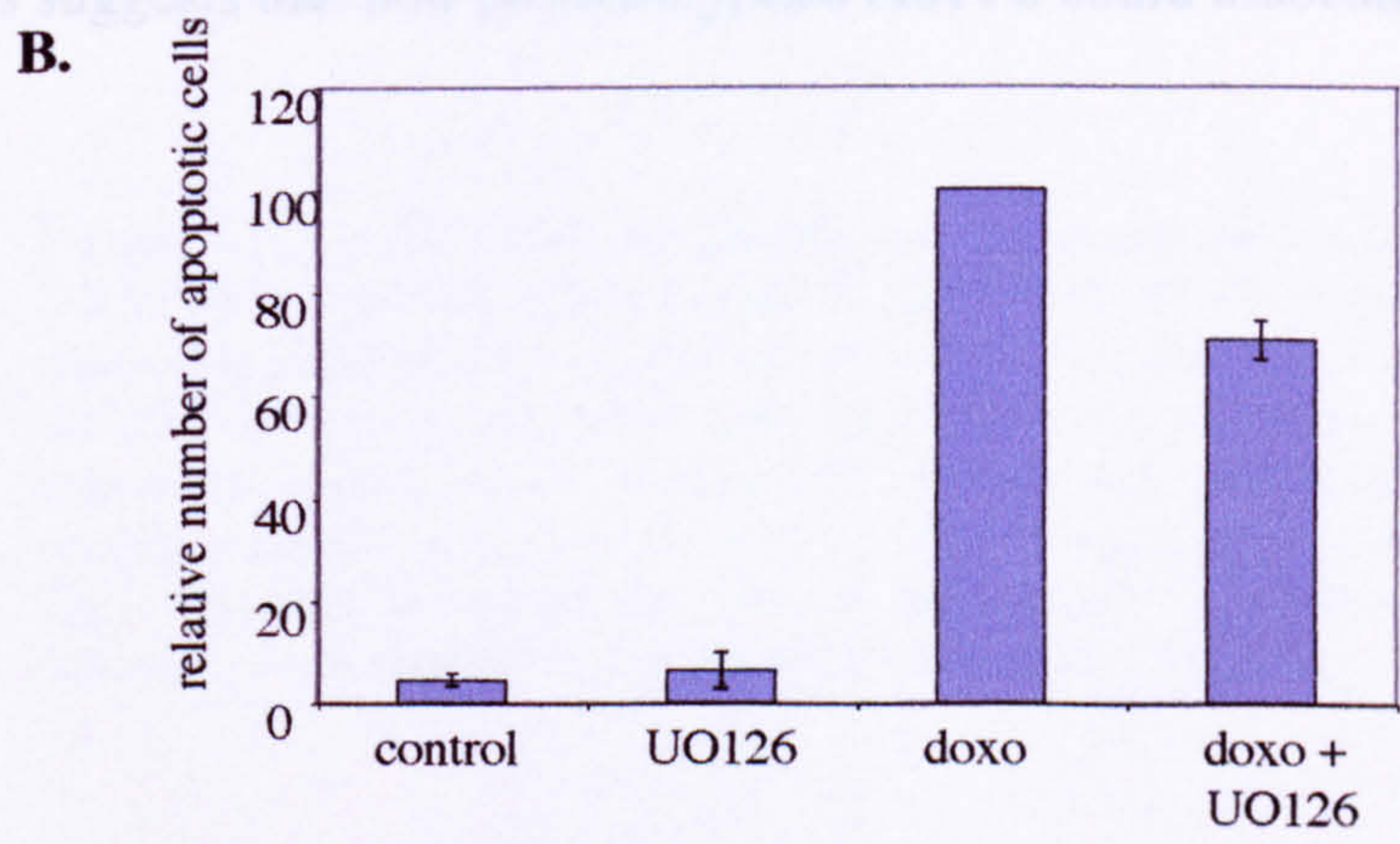
Figure 4.17 MAPK inhibitor UO126 reduces doxorubicin-induced apoptosis in MCF7 cells. MCF7 cells were treated with 4mM doxorubicin (doxo) and 20 \mu M UO126 for 24 hours as indicated. The floating and adhering cells were fixed, stained with propidium iodide and analyzed by FACS. (A) Histogram plot showing the cell cycle profile of MCF7 cells. The percentage of apoptotic cells was measured by accumulation of cells with a sub-G1 DNA content (cells in M1 region). (B) Bar graph representing the relative percentage of sub-G1 cells. The mean values were derived from two independent experiments.
