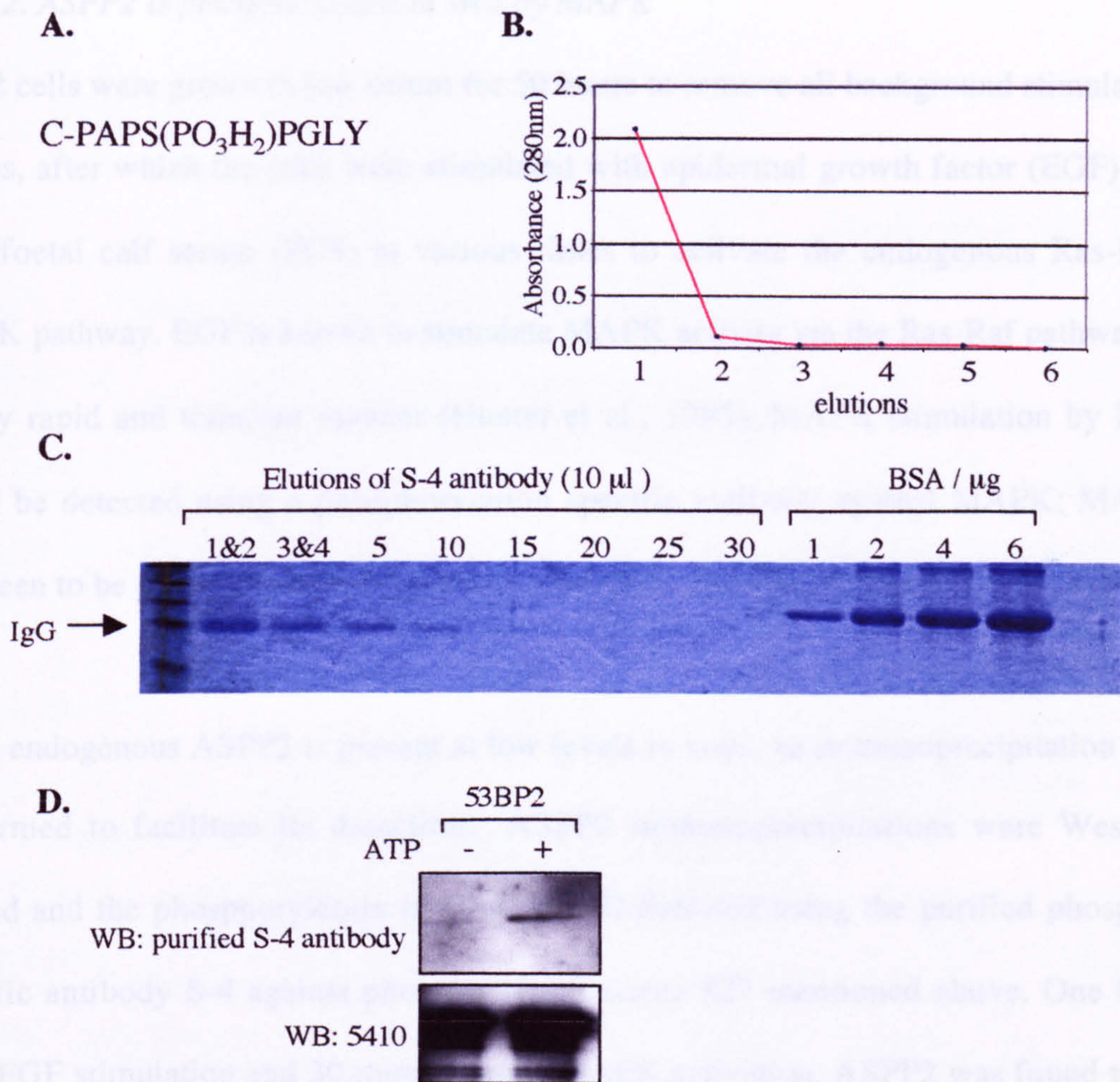
Figure 4.4 S-4 is a phosphospecific antibody that recognizes ASPP2 phosphorylated at serine 827 (A) A phospho-peptide representing amino acids 824-832 of ASPP2 was synthesized with the serine 827 containing a phosphate group. A cysteine was added to the amino-terminus of the peptide. This peptide was used to raise antibodies in mice and rabbit. (B) A polyclonal antibody labelled S-4 raised against the synthetic phosphopeptide was affinity purified with the phospho-peptide column. After adding the serum to the affinity resin column, the column was washed extensively with TTBS. The flow-through of these washes was collected and the protein concentration measured by absorbance at 280nm. After 6 washes all non-specific protein had eluted off the column. The antibody was then eluted with 0.2M glycine (pH 2.8) and neutralized with Tris-HCl (pH 8.0). The first two fractions were pooled and the third and fourth fraction were also pooled. The two pooled sets of eluate were dialyzed with PBS overnight. (C) 10 μl of the two pooled sets of elutions were resolved on an SDS-PAGE gel, as were the eluted fractions 5, 10, 15, 20, 25 and 30. A titration of BSA of known concentration was resolved on the right-hand side of the gel. The protein content of the gel was detected by coomassie blue staining. (D) An in vitro phosphorylation assay was performed on the ASPP2 fragment (693-1128) using recombinant MAPK in the presence or absence of non-radioactive ATP. 300ng of the recombinant GST-ASPP2 fragment was resolved on an SDS-PAGE gel and western blotted with the purified S-4 phospho-specific antibody. Total ASPP2 (693-1128) content was detected by the 5410 antibody.
