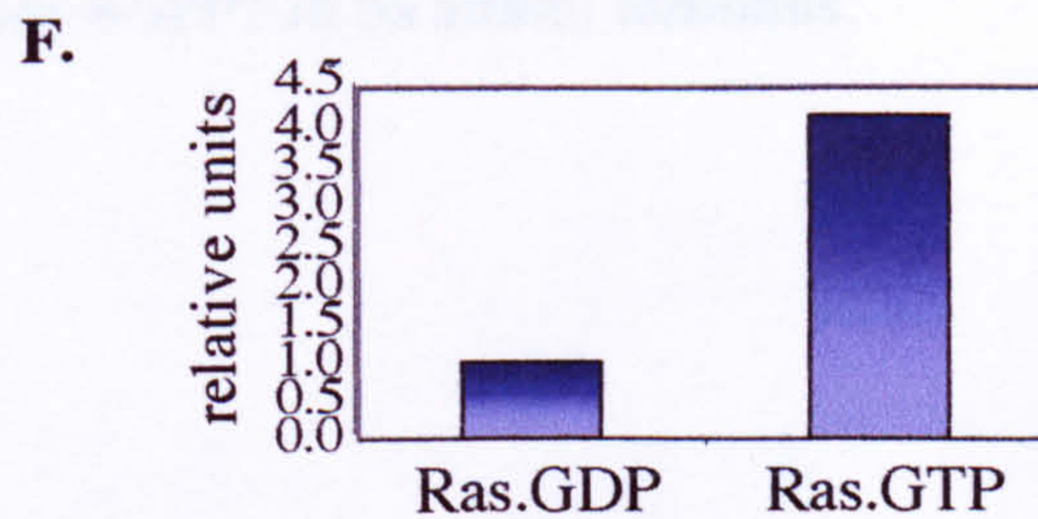
Figure 3.4 Purified amino terminus of ASPP1 binds directly to Ras-GTP with a higher affinity than to Ras-GDP. (A). A plasmid encoding GST-ras was transformed in BL21 cells. Protein expression was induced with IPTG and the protein purified with glutathione beads. GST-ras was eluted from the beads (lane 1). Thrombin was added to GST-ras to cleave the GST tag and aminobenzamide-agarose beads was present to remove the thrombin. An aliquot of the beads containing thrombin and GST is shown (lane 2) as well as the supernatant containing purified ras (lane 3). Ras protein was subsequently dialyzed (lane 4) and concentrated using a centricon column. As expected there was no protein present in the filtrate of the centricon (lane 5) but the ras was concentrated in the remainder of the centricon (lane 6). Aliquots of all stages were resolved on 15% SDS-PAGE gels which was partially transferred onto nitrocellulose. The gel was then stained with gclcode for total protein (A). The four lanes on the extreme right of the gel represents a titration of BSA protein to help approximate the ras concentration at the final step. (B). The nitrocellulose membrane was western blotted for ras using the anti-ras RO2120 antibody. (C). Loading of Ras-GDP and Ras-GTP. Tritium labelled GDP or GTP was added to purified ras at 30°C. To check the efficiency of the ras loading, an aliquot was taken and immunoprecipitated with a ras antibody and washed extensively before being placed on a blot paper in scintillation liquid. The tritium counts are shown in graph (C). Since the tritium counts of the stock GDP and GTP were not equivalent, the moles of GDP and GTP loaded on ras were calculated and shown in (D). (E). Purified ras-GDP or ras-GTP was added to a purified fragment of ASPP1 (1-308) tagged with a V5 epitope. The samples were immunoprecipitated with a V5 antibody and the samples analyzed on an SDS-PAGE gel. A western blot was performed with a Ras antibody and a V5 antibody to check the amount of ASPP1 fragment. As a control, ras-GDP and ras-GTP were immunoprecipitated with V5 in the absence of the ASPP1 (1-308) fragment as shown on the last two lanes. (F). Ras-GTP was immunoprecipitated by ASPP1 (1-308) with a higher affinity than ras-GDP. The signal of the band was quantified and the values shown as a bar graph.
