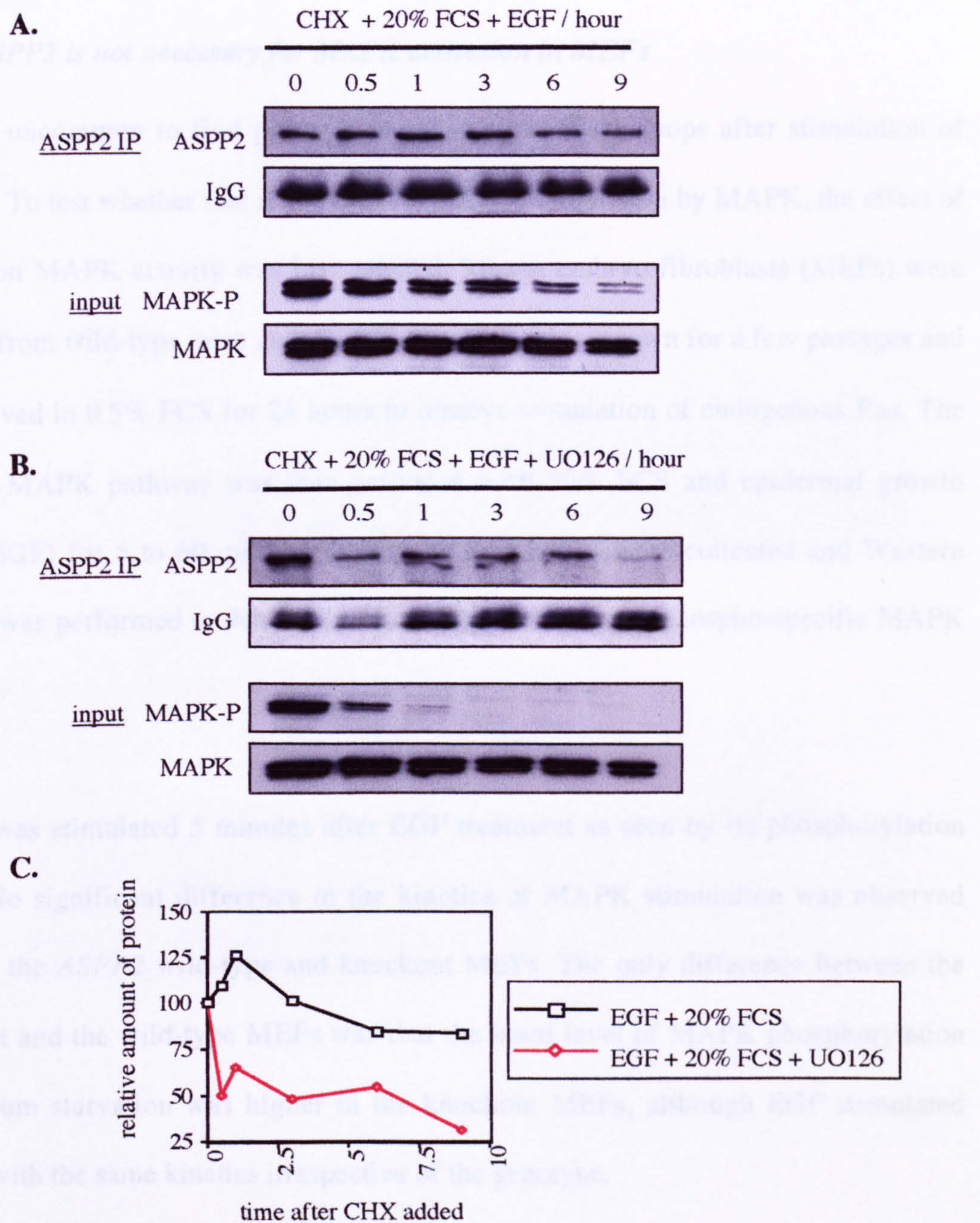
Figure 4.15 MAPK activity is necessary for endogenous ASPP2 stability. MCF7 cells were starved of serum for 24 hours in 0.5% FCS. They were then treated with 50 \mu\text{g}/\text{ml} cycloheximide (CHX) and 20% FCS and EGF, without UO126 (A) or with UO126 (B) for the time indicated. 4mg of lysate was used for immunoprecipitation with the monoclonal 5410 antibody against ASPP2. The immunoprecipitate was western blotted and ASPP2 was detected with the polyclonal bp77 antibody (top panel). The amount of antibody used for the immunoprecipitation was detected with secondary mouse antibody (second panel from the top). 60 \mu\text{g} of input was western blotted and phosphorylated MAPK was detected with phospho-specific MAPK antibody (third panel from the top) and the total MAPK was detected with a MAPK antibody (bottom panel). (C) The intensity of the ASPP2 protein immunoprecipitated was quantified and the bands at 0 hours of CHX addition was set as 100 for both cells.
