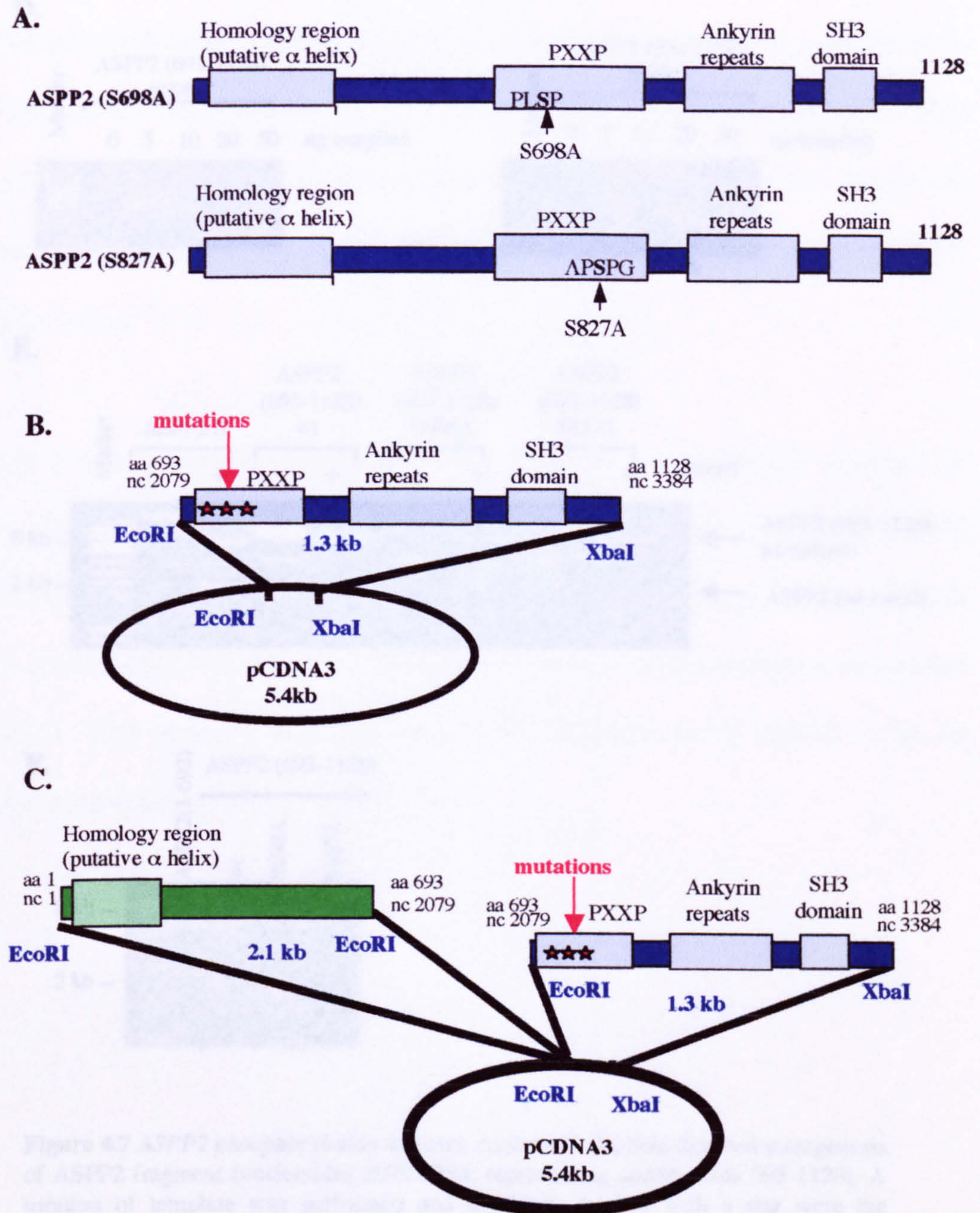
Figure 4.7 Construction of plasmids expressing ASPP2 phosphorylation mutants. (A) Schematic representation of the construction of ASPP2 mutants expression plasmids. The homologous region in the amino terminus is shown, as is the proline rich region (PXXP), the ankyrin repeats and the SH3 domain. The two putative MAPK phosphorylation sites are shown (serine 698 and serine 827). Both of these putative phosphorylation sites were mutated to alanine as described in Materials & Methods. (B) The mutations were introduced by site-directed mutagenesis in the ASPP2 fragment representing amino acids (aa) 693-1128 and nucleotides (nc) 2079-3384. (C) Schematic representation of the ASPP2 amino-terminus fragment (amino acids 1-693, representing nucleotides 1-2079) subsequently added to the mutated carboxy-terminus fragment.
