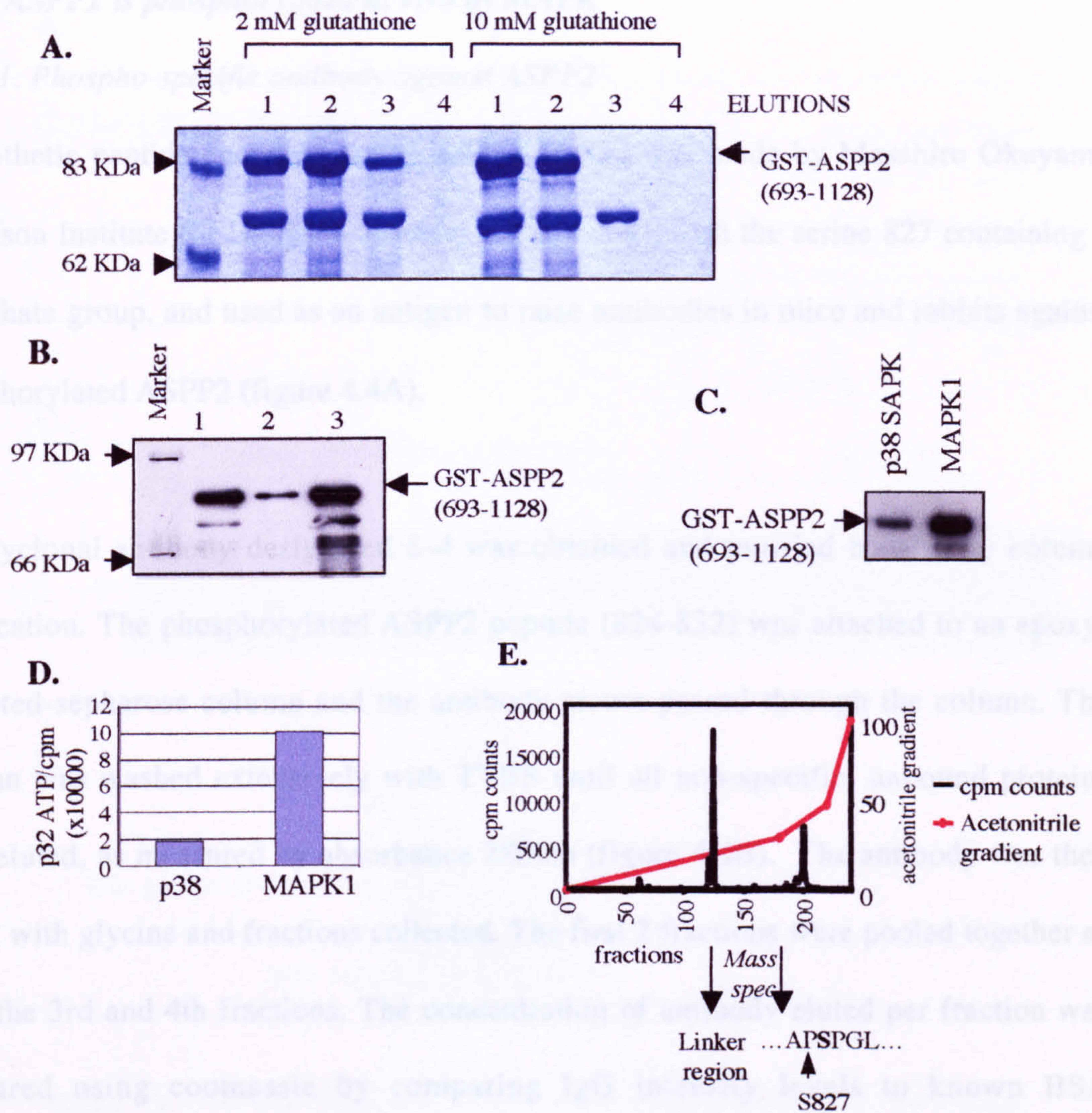
Figure 4.3 ASPP2 is phosphorylated in vitro by MAPK (A) The carboxy terminus of ASPP2 (693-1128) was expressed as a GST-fusion protein in BL21 cells and purified with glutathione sepharose beads. The protein was eluted off the beads using glutathione at either 2mM or 10mM and the samples were collected after each of the four washes with glutathione (labelled 1-4). An aliquot was collected, run on an SDS-PAGE gel and the total amount of protein was detected by coomassie staining. Samples 1,2 and 3 from 2mM glutathione and 1 and 2 from 10mM glutathione were pooled and dialyzed in water. The protein was then concentrated and resuspended in 1x kinase buffer. (B) The pooled samples were analyzed by western blotting before (1) and after (3) dialysis and GST-ASPP2 (693-1128) was detected with a 5410 antibody against the carboxy-terminus of ASPP2. An aliquot of elution 3 from 10mM glutathione shown in (A) was run on lane 2. (C) An in vitro phosphorylation assay was performed with ^{32}\text{P} labelled ATP as described in Materials and Methods with the recombinant ASPP2 fragment in the presence of recombinant p38 SAPK or MAPK. The phosphorylated ASPP2 fragment was resolved on an SDS-PAGE gel, transferred onto nitrocellulose and the ATP levels detected by autoradiography. (D) The intensity of the phosphorylated ASPP2 fragment was measured using the GeneTools from SynGene programme and represented on a bar graph. (E) The MAPK phosphorylated ASPP2 fragment was trypsinized and chromatographed on a Vydac \text{C}_{18} column (E, bottom panel). The radioactive peptides were measured by mass spectrometry. The first peak was shown to represent the GST linker region whereas the second represented a region of equal mass to the fragment containing the serine 827.
