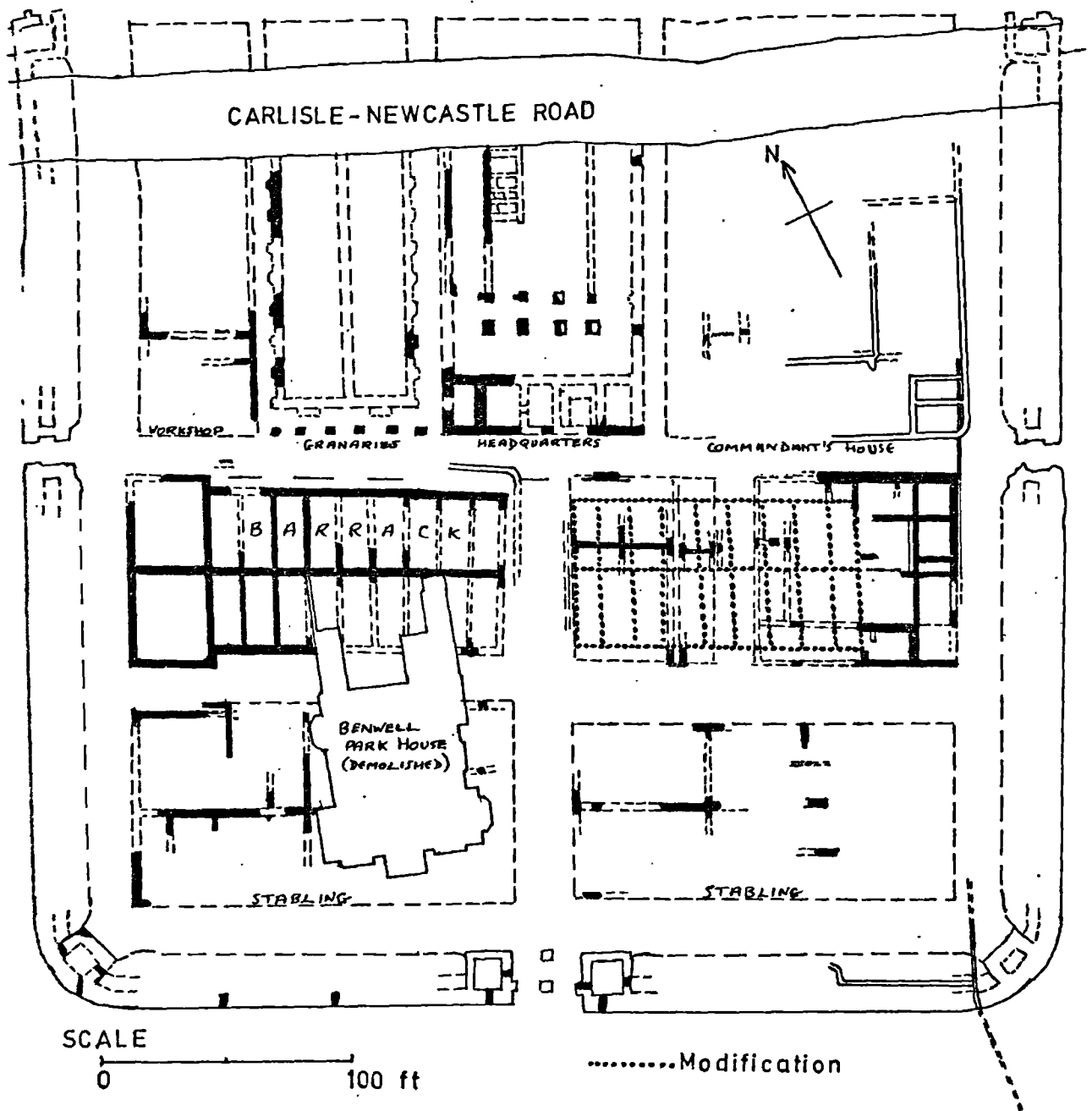
Figure I. Suggested revision of the plan of Benwell fort in the Hadrianic period. (Plan after F.G.Simpson and I.A.Richmond)
